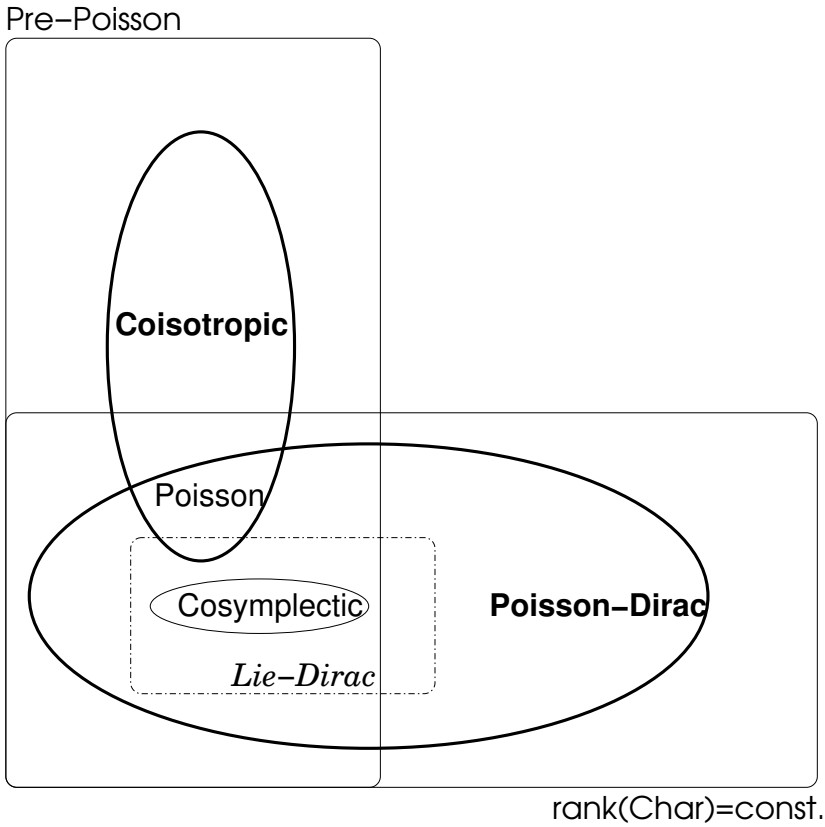
Fig. 1 Relation between the classes of submanifolds considered in this note. Recall that a submanifold N is Pre-Poisson iff rank(\sharp TN^\circ + TN) = const. and that char(N) = \sharp TN^\circ \cap TN .
