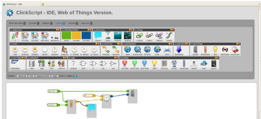
Fig. 5.8 Using the Clickscript Mashup Editor to Create a Physical Mashup by Connecting Building Blocks Directly to a Browser
