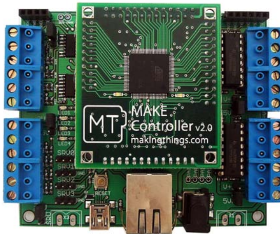
Fig. 4.2 The Make Controller Kit v2.0 Assembled with Controller and Application Boards 56
