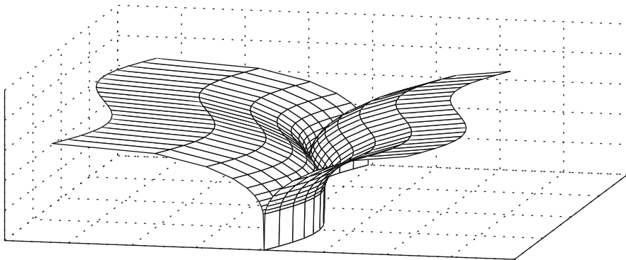
Fig. 9.3 The exponent p with a ridge
