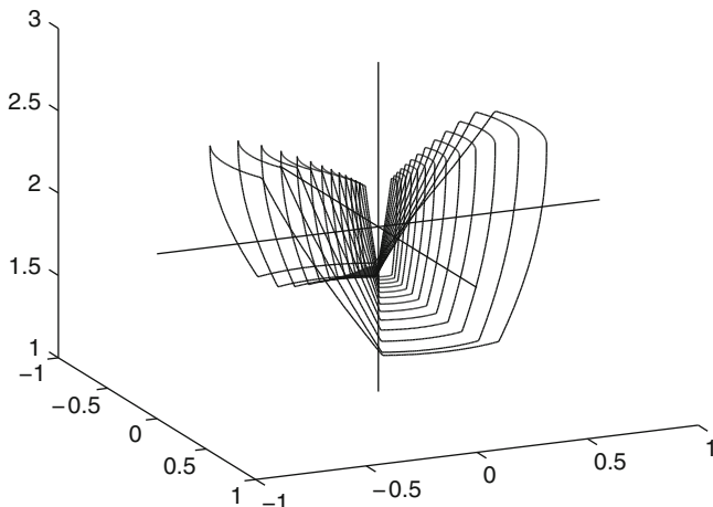
Fig. 11.1 A contour sketch of the exponent p
