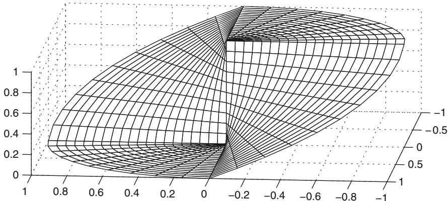
Fig. 9.1 A function which cannot be approximated by a continuous function
