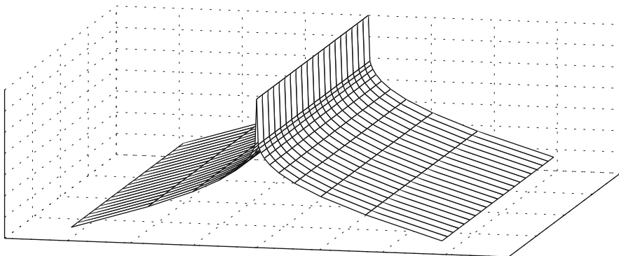
Fig. 9.4 The exponent p with a through
