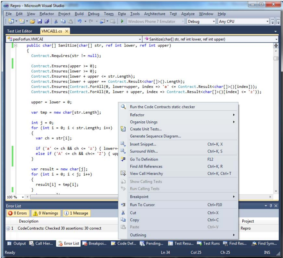
Fig. 2. A screenshot illustrating the user experience with Clousot in Visual Studio. The user can run the analyzer on the whole project, or she can opt for a selective method/class verification with a simple right click. The output is reported in the usual ErrorList window, the same where e.g. the compiler provides its output.
