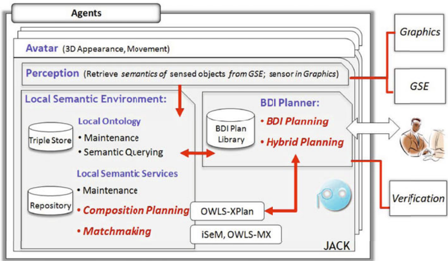
Fig. 6. ISReal user agent architecture
