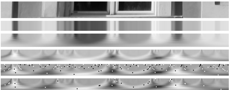
Fig. 2. From top to bottom: sampled rectangle next to a line segment, collapsed profile, Gaussian scale space with 6 octaves and 5 scales per octave, DoG scale space, extrema (white and black dots) in DoG scale space, accepted feature points with refined positions in DoG scale space
