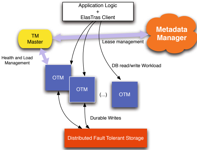
Fig. 1. ElasTraS architecture
