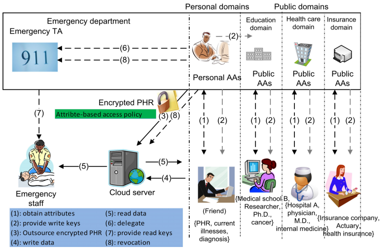
Fig. 1. The proposed multi-owner, multi-authority, and multi-user framework for access control of PHR in cloud computing
