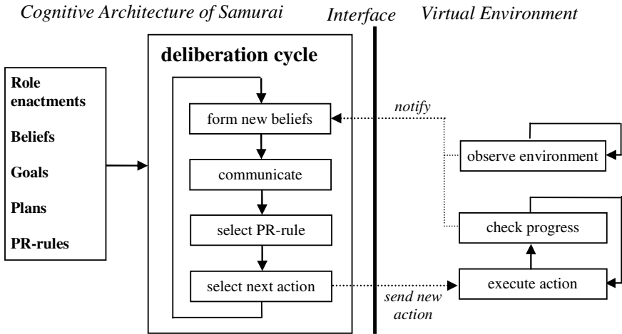
Fig. 1. Cognitive architecture and interaction with Virtual Environment
