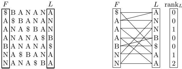
Fig. 1. BWT matrix \mathcal{M} and inverse BWT permutation for text S = BANANA\$
