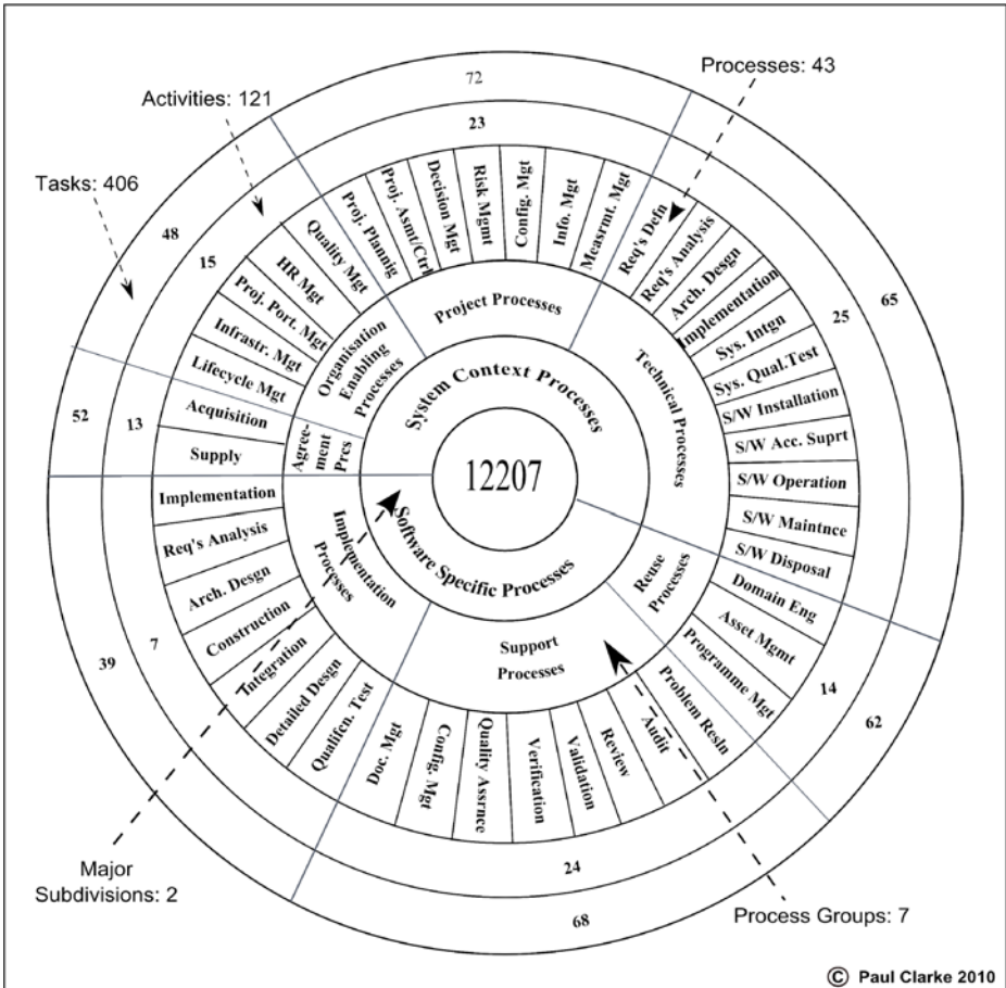
Fig. 2. ISO/IEC 12207 Topology
