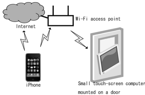
Fig. 2. Hardware configuration of the prototype
