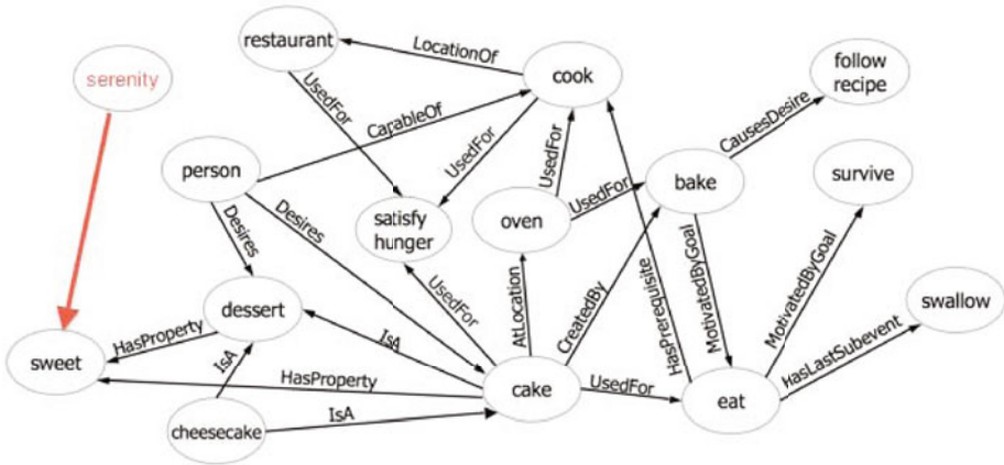
Fig. 1. A sketch of AffectNet
