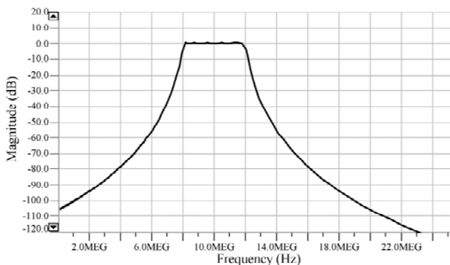
Fig. 9. Magnitude response of the 6 th order Chebyshev complex TT biquad filter
