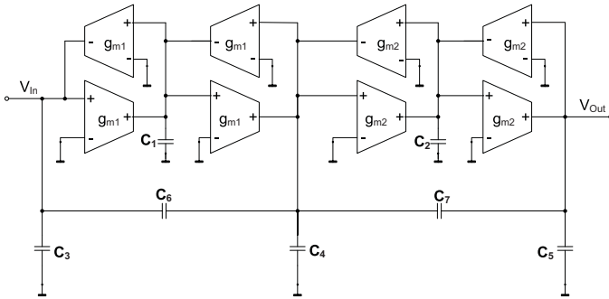
Fig. 4. The Gm-C lowpass ladder filter
