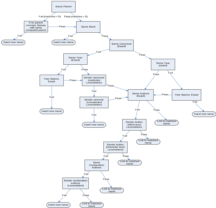
Fig. 4. Example decision tree & matching process
