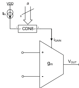
Fig. 5. The schematic of the Programmable Gain OTA
