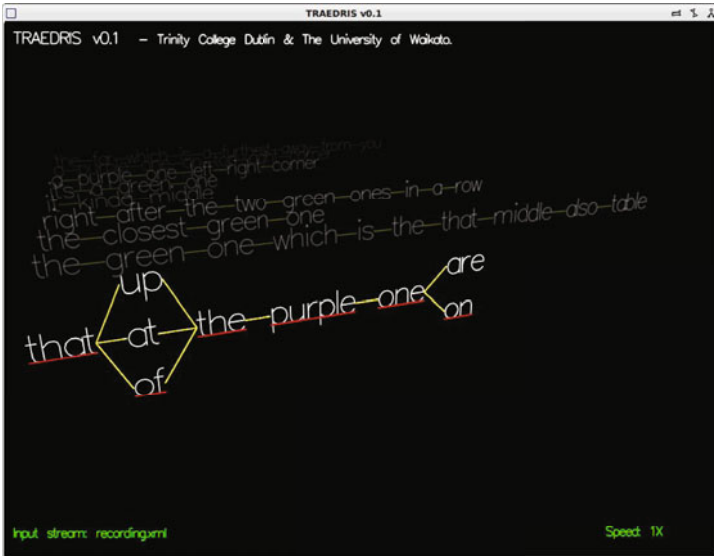
Fig. 2. TRAEDRIS user interface
