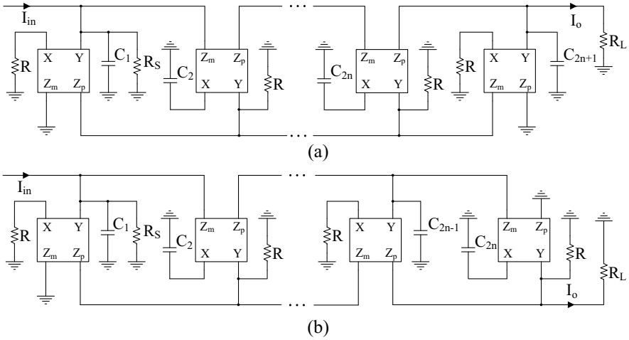
Fig. 4. The (a) odd and (b) even order low pass state variable leap-frog filter
