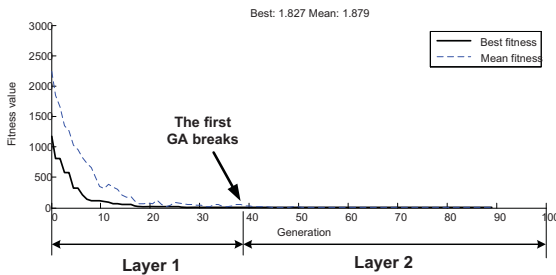
Fig. 12. Evolution of the best fitness and the mean fitness values vs. generations for Application 3
