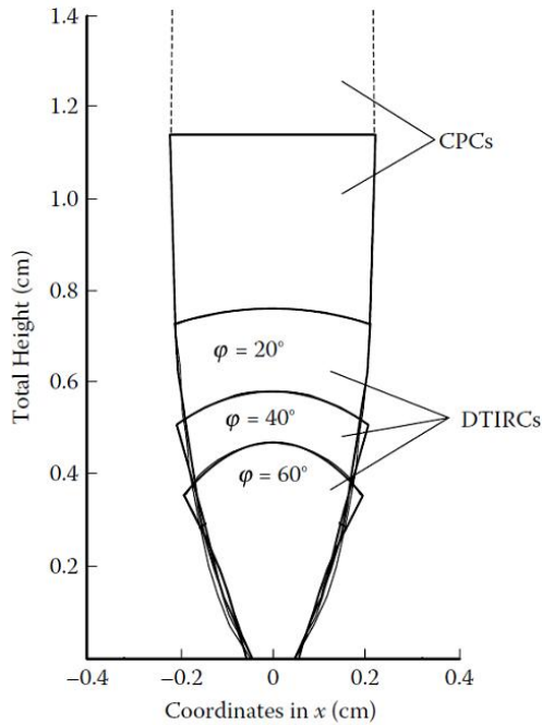
Fig. 4. Comparison of three DTIRCs with different arc angle and a CPC [8]
