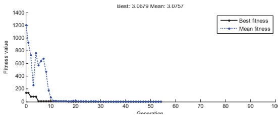
Fig. 10. Evolution of the best fitness and the mean fitness values vs. generations for Application 2
