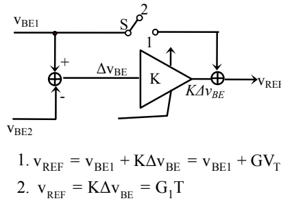
Fig. 1. Principle for a PTAT (2) or a bandgap (1) reference
