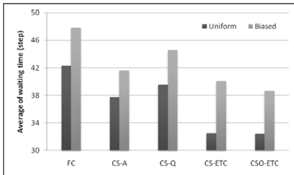
Fig. 6. Comparison of traffic controllers on the destination distribution (uniform and biased distributions)
