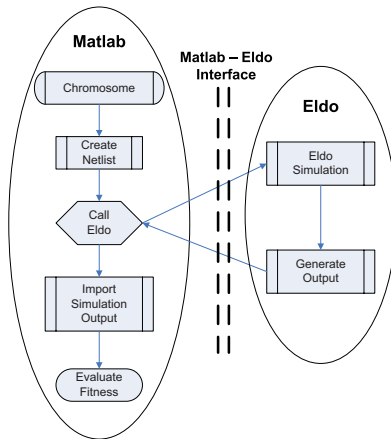
Fig. 2. The evaluation of the fitness function over the Matlab-Eldo interface
