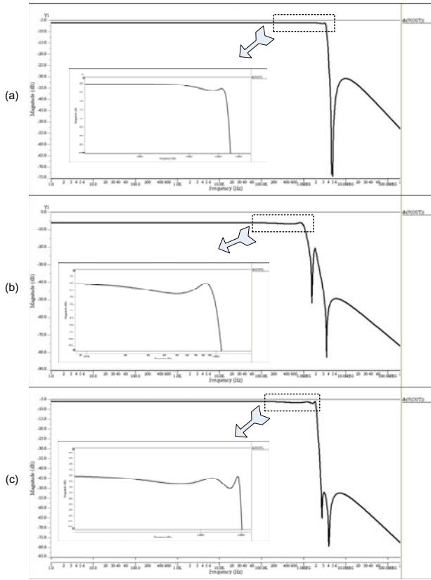
Fig. 8. The Gm-C filter characteristic in the (a) 2^{nd} generation, (b) 14^{th} generation, (c) final generation
