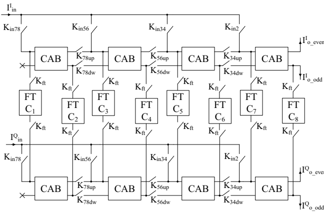
Fig. 2. The proposed FPAA block diagram
