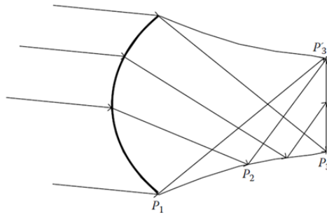
Fig. 3. General design of a DTIRC [7]
