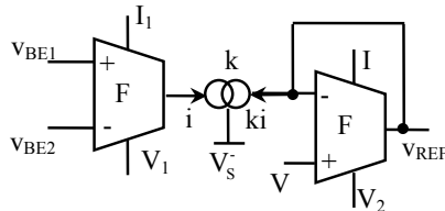
Fig. 2. Block diagram for bandgap voltage references with nonlinear transconductors
