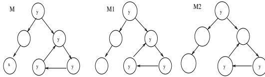
Fig. 2. Updating (M, s) with AG\neg x \vee AF\neg y
