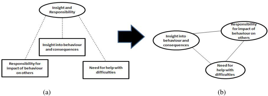
Fig. 2. (a) Sample fixed generic component from GRiST knowledge structure and (b) its MRF equivalent structure
