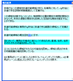
Fig. 4. Extraction window
