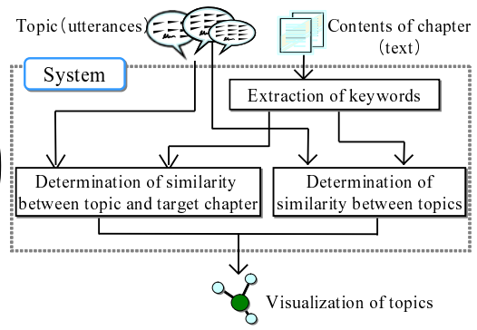
Fig. 2. Processing steps
