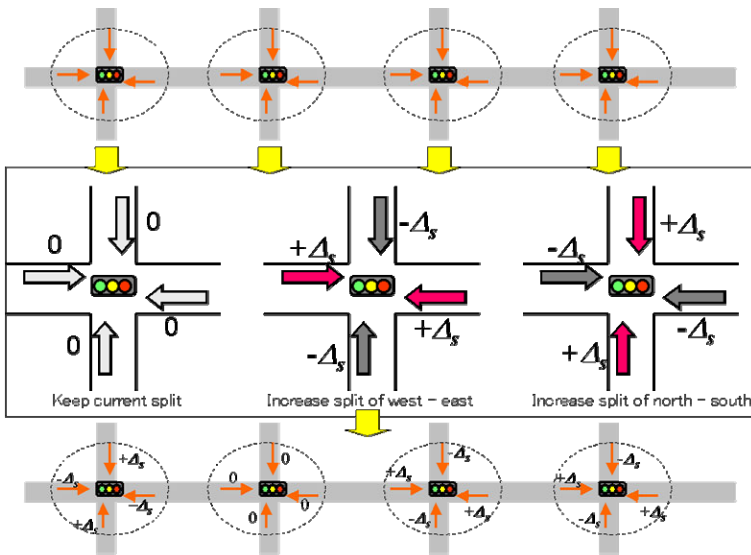
Fig. 3. Split adjustment
