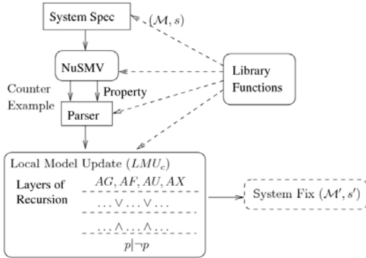
Fig. 3. Implementation graph
