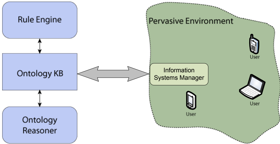
Fig. 1. Architectural overview
