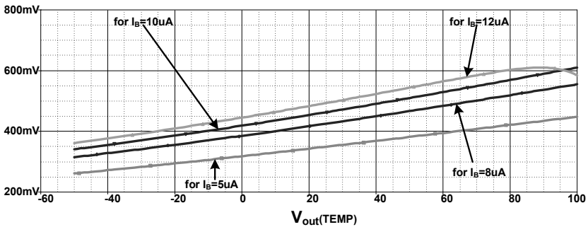
Fig. 5. PTAT reference realized with the circuit in Fig.4,a having input of M5 grounded
