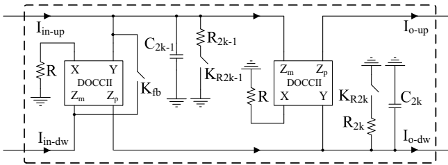
Fig. 6. The proposed CAB architecture
