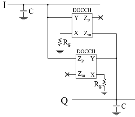
Fig. 7. The linear frequency translation circuit
