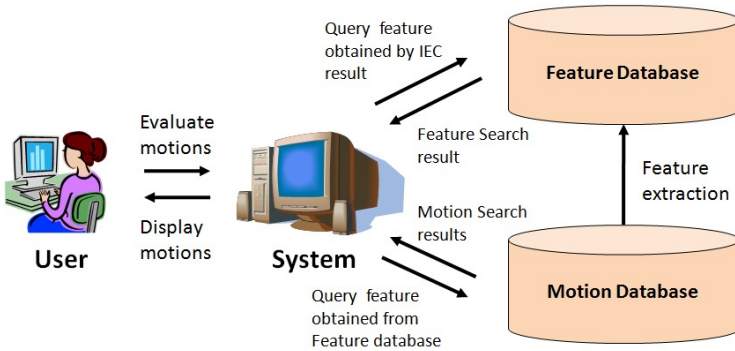
Fig. 3. Overview of motion retrieval system
