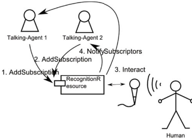
Fig. 2. Perception event subscription
