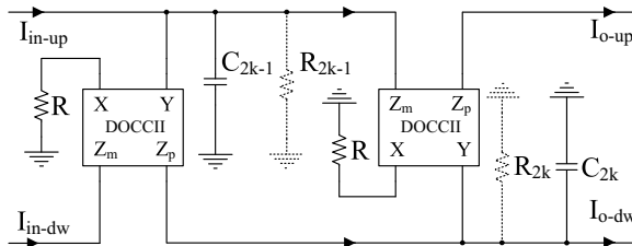
Fig. 5. A second order section in leap-frog filters
