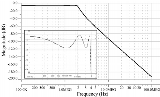
Fig. 8. Magnitude response of the 5 th order Chebyshev leap-frog filter
