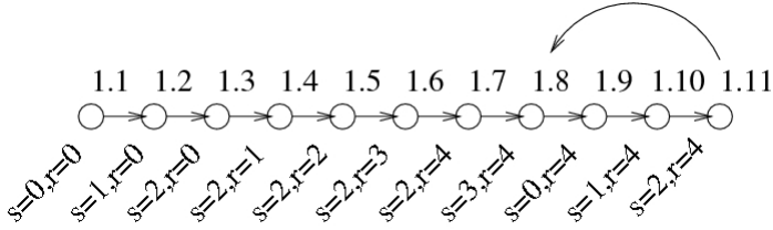
Fig. 7. local model for window size n = 5 . s represents s.sentId and r r.receivedId .
