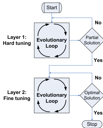
Fig. 6. The double-layer Genetic Algorithm structure
