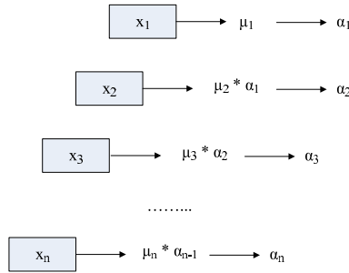
Fig. 1. Temporal information processing over a tree branch
