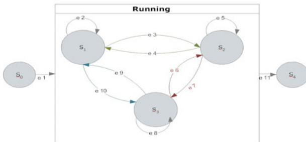
Fig. 1. State machine diagram (the boxes indicate states and the arrows represent transitions)
