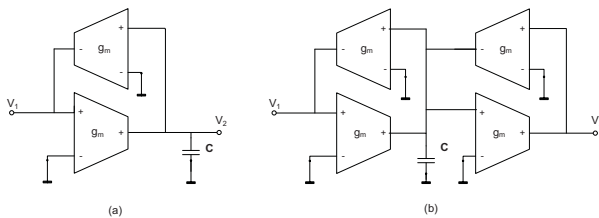
Fig. 3. Gm-C simulation of (a) grounded inductor (b) floating inductor
