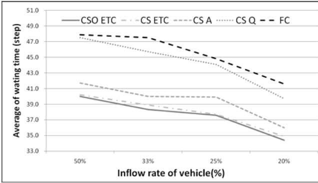
Fig. 7. Comparison of traffic controllers on the inflow rate (50%,33%,25%, and 20%)
