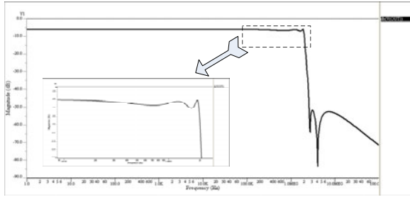
Fig. 11. The Gm-C filter characteristic after fine-tuning
