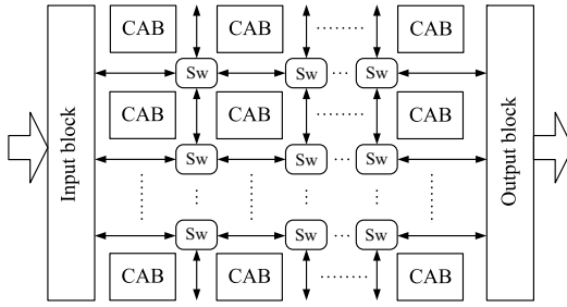
Fig. 1. The General Architecture of a FPAA
