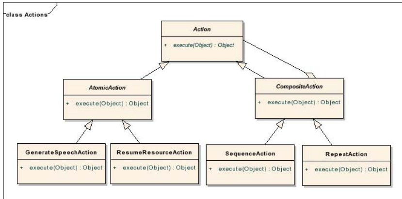
Fig. 3. Actions hierarchy
