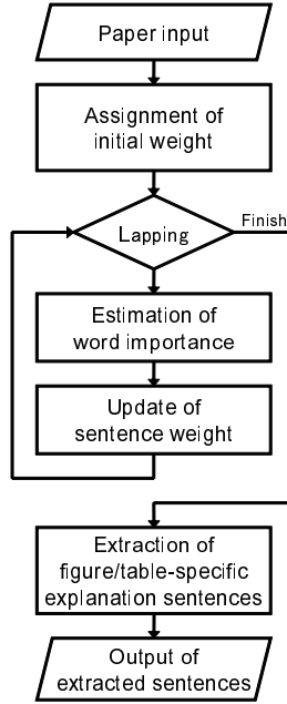
Fig. 2. Processing flow
