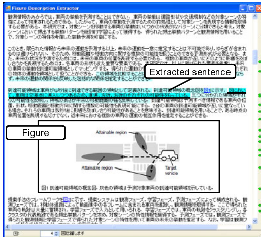
Fig. 3. Main window
