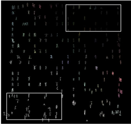
(a) SOM layout of motion database colored by Effort feature: Red assigned to the Weight feature value and green assigned to the Space feature value and blue assigned to the Time feature value.
