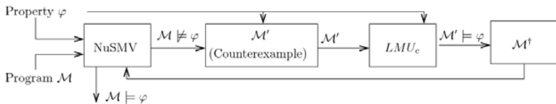
Fig. 2. Process graph of \text{lmuc}
