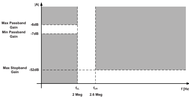
Fig. 7. The filter design specifications
