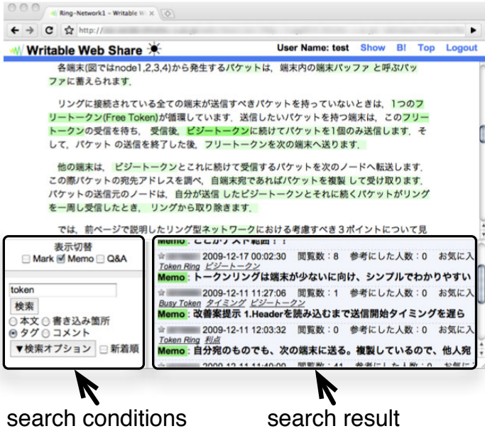
Fig. 3. Searching function
