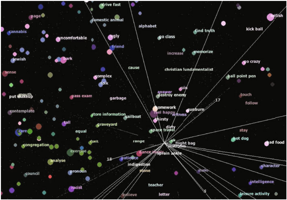
Fig. 4. Navigating SenticSpace
