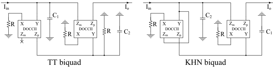
Fig. 3. The TT and KHN second order sections based on DOCCII-s
