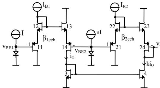
Fig. 3. BVR with gate coupled composite CMOS pairs
