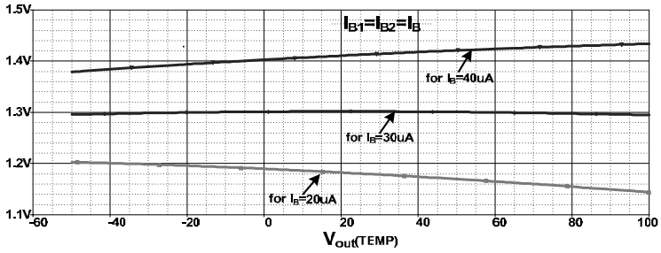
Fig. 6. Output control by IB for a BVR including an offset
