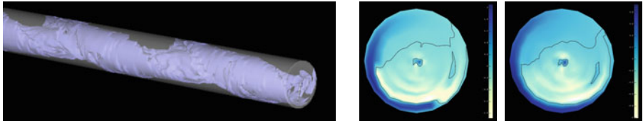
(a) Path line oriented topology in complete time-dependent field. Third dimension used to stack time steps ( 60 < t < 80 visible). Isosurface encloses attracting behavior. (b) Path line oriented topology (left) compared to divergence (right) for t = 70 . Colormap and zero isolines divide the field into areas with converging (negative values) and diverging behavior (positive values)
