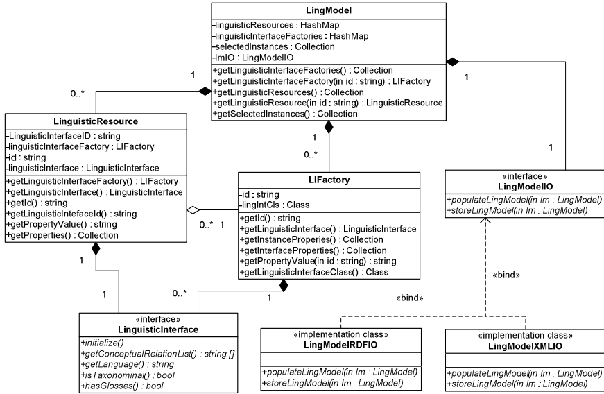
Fig. 6 Class diagram of the main components of LW model
