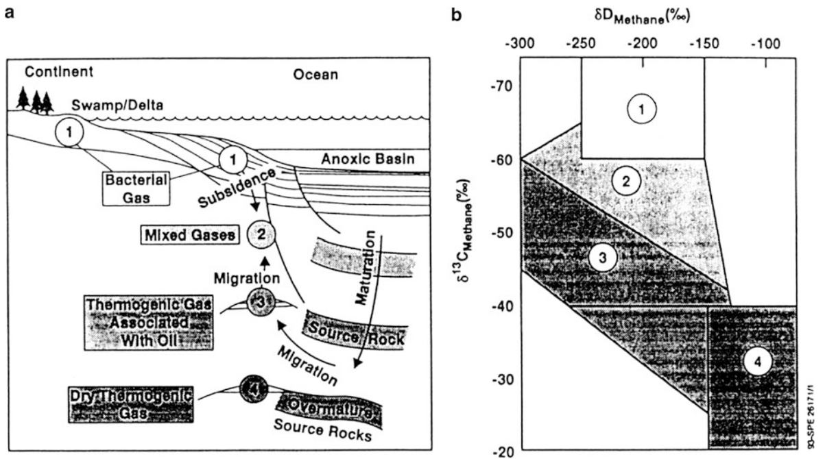
Fig. 31.18 Schoell plot showing relationship between C and H isotope ratios of natural gas samples and depth of generation (Reproduced from Schoell 1983 with permission of AAPG & and whose permission is required for further use)
