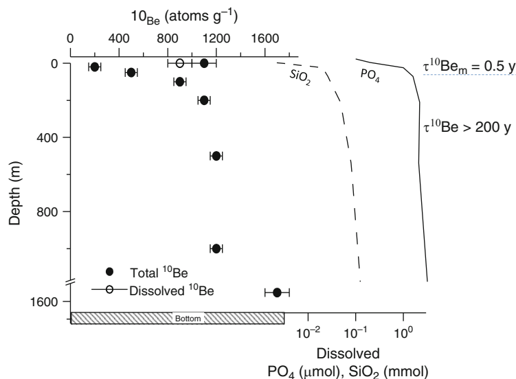
Fig. 5.4 ^{10}\text{Be} , phosphate, and silica concentrations in the water column in the San Nicolas Basin (Kusakabe et al. 1982). Above the thermocline in the “mixed layer” (upper \sim 100 m), high concentrations of suspended particles cause rapid removal of
