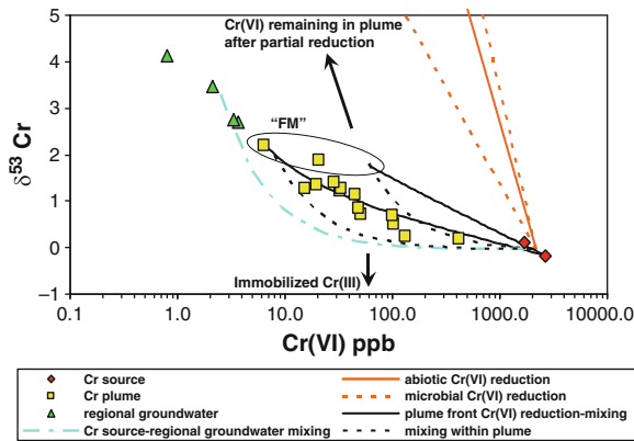
Fig. 10.3 \delta^{53/52}\text{Cr} and \text{Cr(VI)} concentration data for groundwater at the Hinkley, CA site “Cr source” samples were collected at the PG&E compressor facility, “Cr plume” samples were collected downgradient of the compressor facility within the \text{Cr(VI)} plume. “Regional groundwater” samples were collected just upgradient, just down gradient, and well away from the plume. The “Cr source-regional groundwater mixing” curve shows mixing between Cr source and average regional groundwater. The “abiotic \text{Cr(VI)} reduction vector” is from Ellis et al. (2002); the “microbial \text{Cr(VI)} reduction” vectors are from Sikora et al. (2008), and show the range of fractionation observed in their experiments. The field labeled “FM” represents plume Front and Margin samples produced through combined \text{Cr(VI)} reduction and advective mixing with regional groundwater as described in the text. The “mixing within plume” curves show mixing between “FM”-type and “Cr source” groundwaters. The arrow labeled “ \text{Cr(VI)} remaining in plume following partial reduction” shows the direction that homogeneous \text{Cr(VI)} reduction within the plume will move residual \text{Cr(VI)} compositions on this diagram. The arrow labeled “immobilized \text{Cr(III)} ” shows that \text{Cr(III)} produced during \text{Cr(VI)} reduction will have negative \delta^{53/52}\text{Cr} . The uncertainty of the data for all samples is less than the size of the symbol
