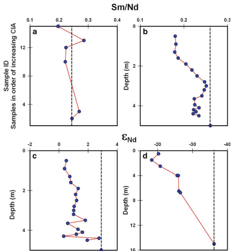
Fig. 26.5 The behavior of Sm/Nd and \epsilon_{Nd} during chemical weathering as recorded in soil profiles. The results show different patterns. (a) (Toorango granodiorite, Australia; Nesbitt and Markovics 1997) indicates Sm/Nd remain nearly constant during weathering; whereas (b, c) (Neogene basalts from South China; Ma et al. 2010) and (d) (granodiorite from southern Cameroon; Viers and Wasserburg 2004) depict effects of preferential mobilization of Sm. The bottom and top sides of the figures show the least and most weathered rocks; the dashed straight line in the figure represents the bed rock value
