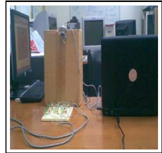
Fig. 4. Experimental setup: Receiver is Web camera, Transmitters are LEDs on Breadboard
