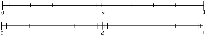
Fig. 2.13 Bakhvalov mesh (top) and Shishkin mesh (below) for a reaction-diffusion problem with an internal layer on both sides of x = d
