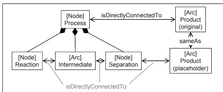
Fig. 4.27: Alternative 3 – duplication of the arc ; correspondence is established via the sameAs relation
