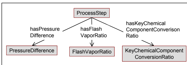
Fig. 8.12: Exemplary property assignment to process step
