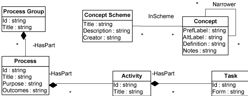
Fig. 3. A model of 12207 and 24765 semantic wikis
