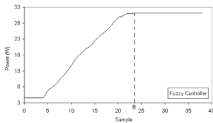
Fig. 8 Sample vs Power of PV array using Fuzzy Controller method B. The Fuzzy Controller’s method reaches MPP after the 24 th iteration.
