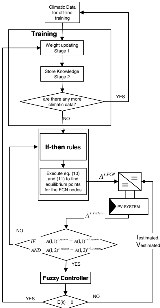
Fig. 10 Simplified flowchart of the proposed method
