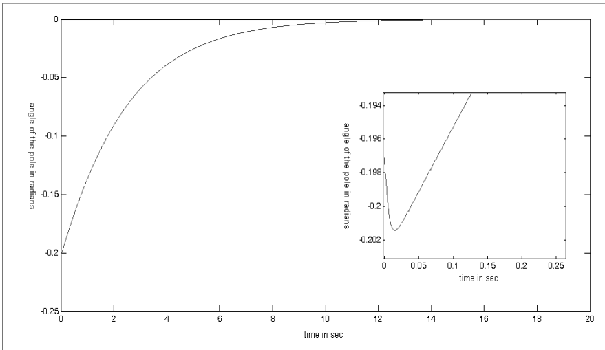
Fig. 15 State x_1(t) for initial condition x_1(0) = -\pi/16, x_2(0) = -\pi/4
