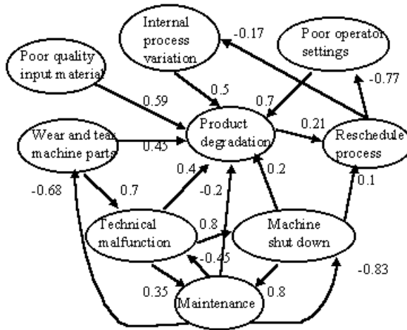
Fig. 5 Supervisor- Fuzzy Cognitive Map with weights
