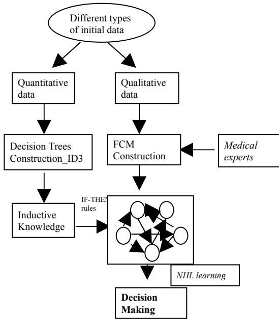
Fig. 6 The decision making system constructed by Decision Trees and Fuzzy Cognitive Maps
