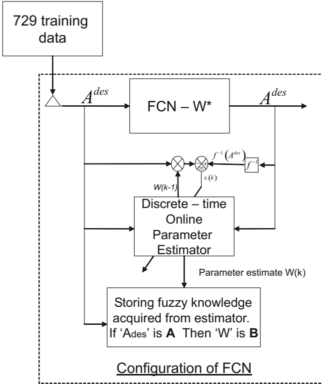
Fig. 10 Off line training of the FCN with data from the physical system
