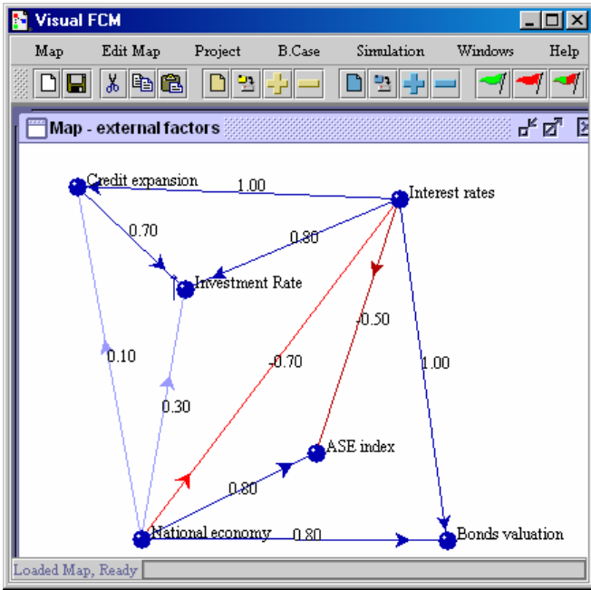
Fig. 19 External factors concepts map
