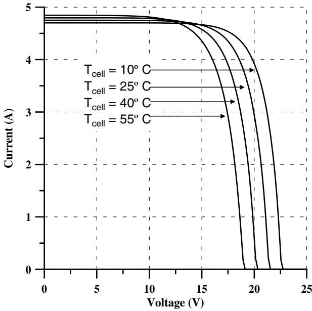
Fig. 3 PV array I-V Characteristics at various Cell Temperatures
