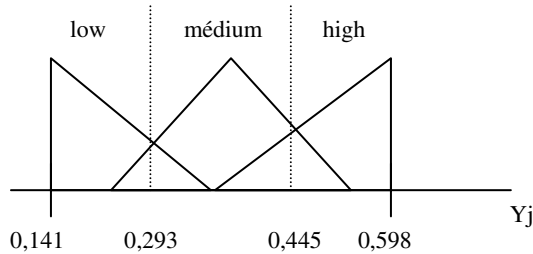
Fig. 15 Fuzzy sets for Exposition to organizational factors
