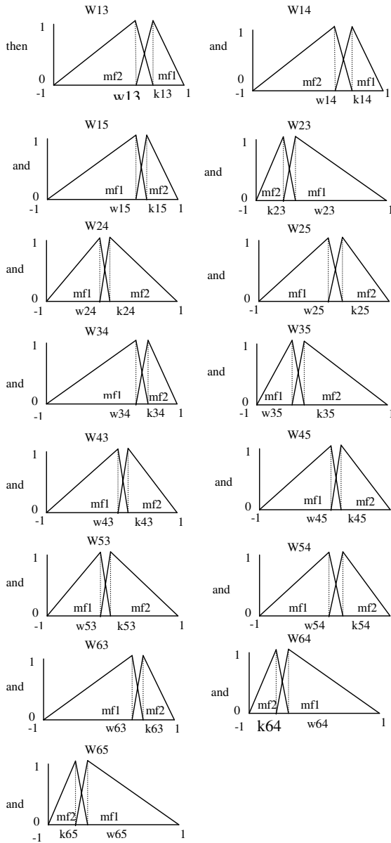
Fig. 12 Right hand side (Then part)
