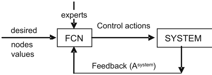
Fig. 24 FCN in close interaction with the system
