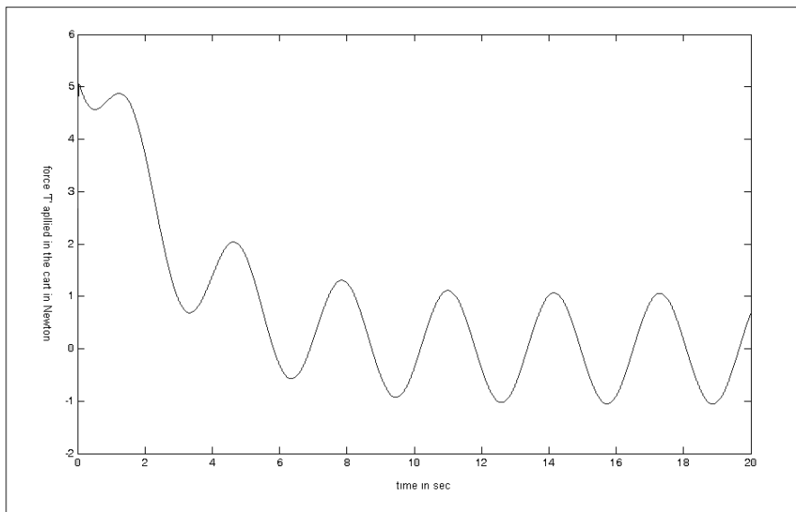
Fig. 21 Force T applied in the cart for tracking state x_1(t) in the desired value \frac{\cos(2\pi t)}{16} for initial condition x_1(0) = -\pi/8, x_2(0) = \pi/16
