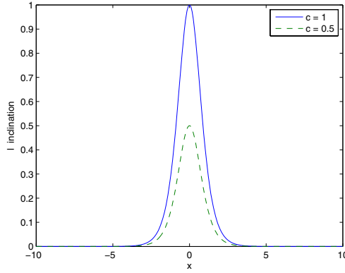
Fig. 4 Inclination of sigmoid function f = \tanh(c_l x) when c_l = 1 and c_l = 0.5 respectively
