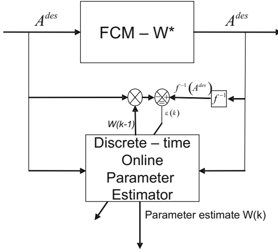
Fig. 6 Online parameter estimator designed for FCMs
