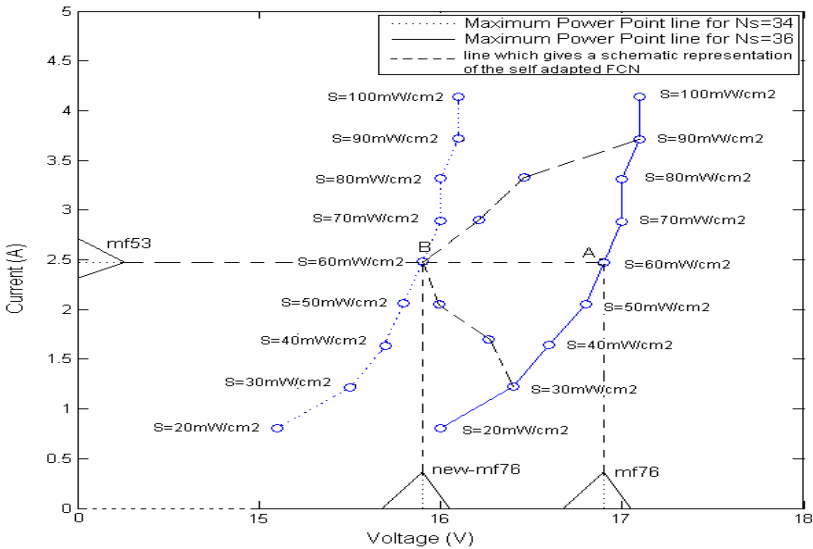
Fig. 16 MPP lines corresponding to the temperature of 25^\circ\text{C} and different insolation values for the BP270L PV model
