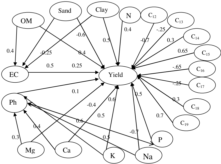
Fig. 7 FCM model for describing the final cotton yield
