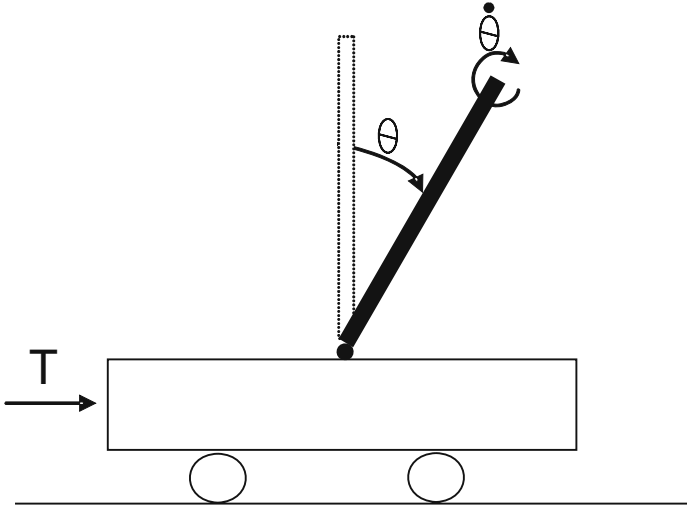
Fig. 8 Inverted Pendulum
