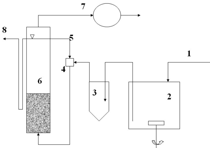
Fig. 22 Schematic representation of the pilot plant used for anaerobic wastewater treatment: 1) Raw wastewater, 2) Acidification tank, 3) Sedimentation tank, 4) pH conditioning tank, 5) Recycle stream, 6) UASB reactor, 7) Biogas measurement and analysis, 8) Treated effluent
