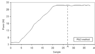
Fig. 7 Sample vs Power of PV array using P&O method A. The P&O method reaches the MPP for the first time after the 27 th iteration.
