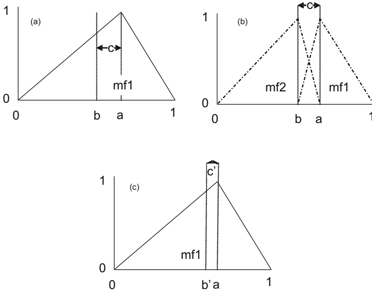
Fig. 11 Conditions for creating new triangular membership function. (a) Present triangular membership function with pick corresponding to the value a of the variable, (b) c > \text{specified threshold} (creation of new triangular) and (c) c < \text{specified threshold} (non-creation of new triangular)
