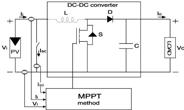
Fig. 6 Step-up boost converter for MPPT
