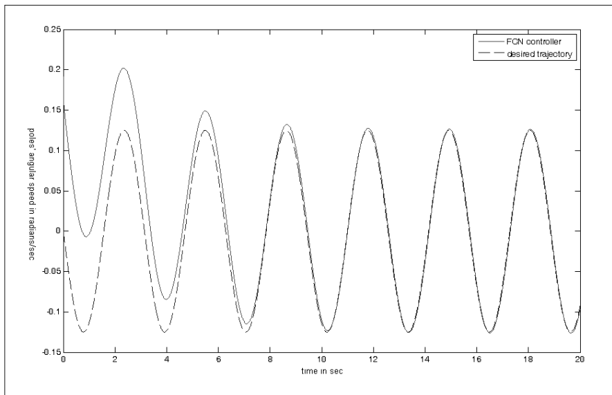
Fig. 20 State x_2(t) and its desired value -\frac{\sin(2\pi t)}{8} for initial condition x_1(0) = -\pi/8, x_2(0) = \pi/16
