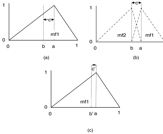
Fig. 13 Creation of new triangular membership function: (a) present triangular, (b) c > specified threshold (creation of new triangular), (c) c < specified threshold (non creation of new triangular)
