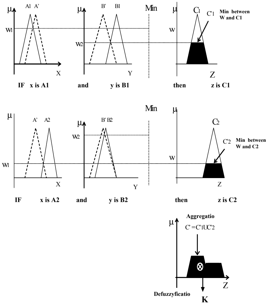
Fig. 7 Approximate reasoning
