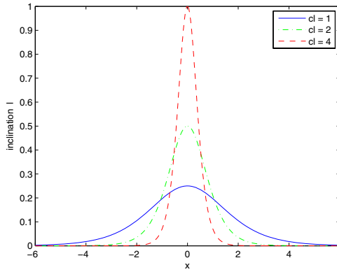
Fig. 2 Inclination of sigmoid function f = \frac{1}{1+e^{-c_l x}} when c_l = 1, 2, 4
