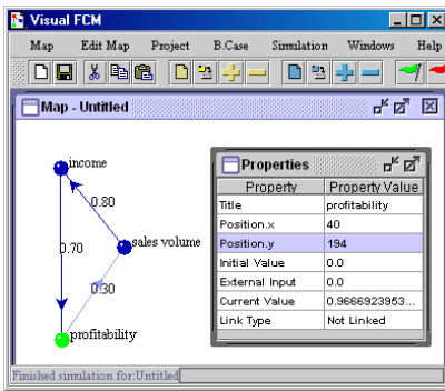
Fig. 7 Sample FCM calculations with feedback loop
