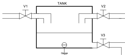
Fig. 1 Process control problem
