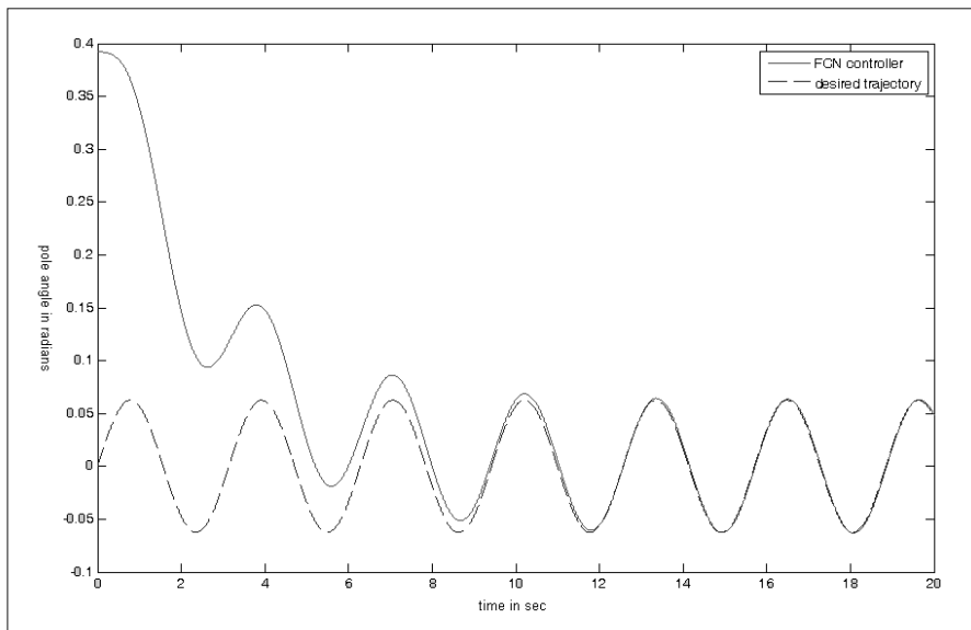
Fig. 16 State x_1(t) and its desired value \frac{\sin(2\pi t)}{16} for initial condition x_1(0) = \pi/8, x_2(0) = 0
