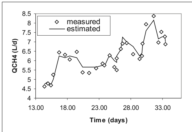
Fig. 27 A comparison between estimated and measured Q_{CH_4} values for the experimental anaerobic digestion process
