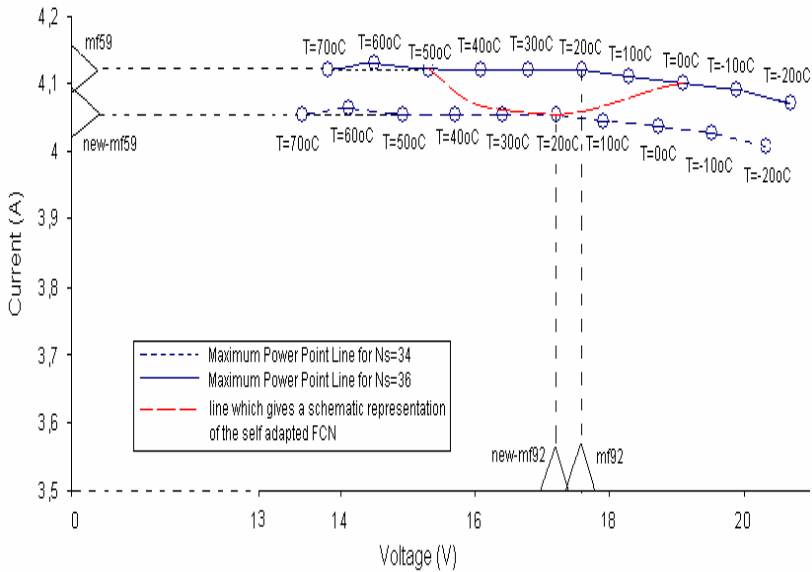
Fig. 17 MPP lines corresponding to the insolation of 100\text{mW}/\text{cm}^2 and different temperature values for the BP270L PV model
