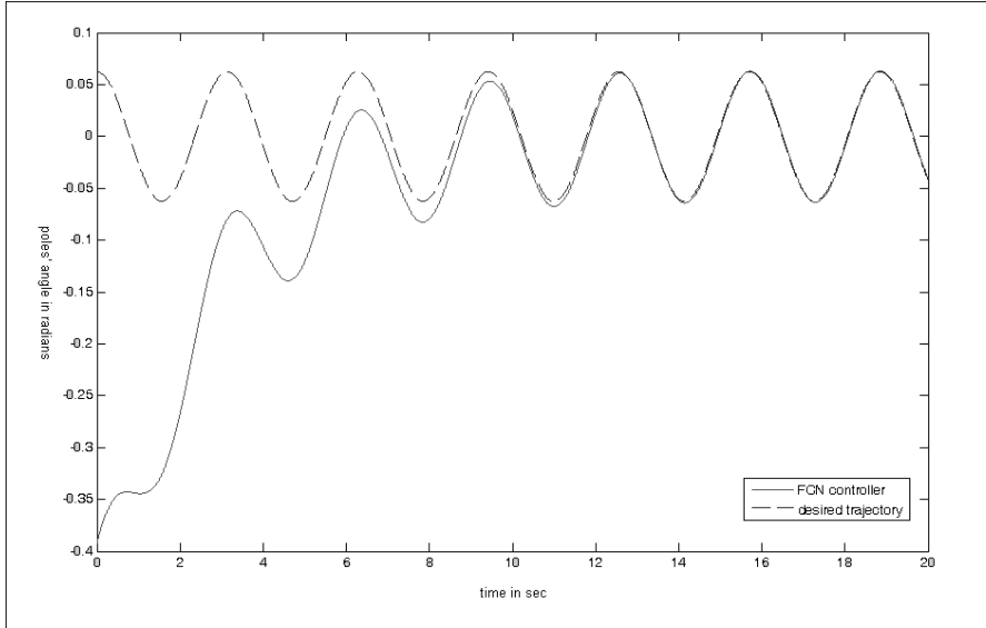
Fig. 19 State x_1(t) and its desired value \frac{\cos(2*t)}{16} for initial condition x_1(0) = -\pi/8 , x_2(0) = \pi/16
