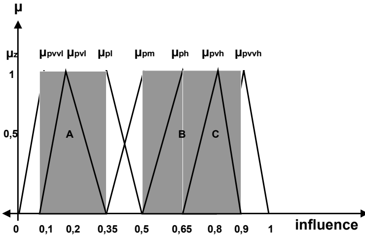
Fig. 5 Linguistic assignments
