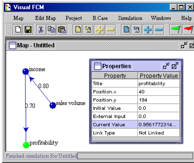
Fig. 6 Sample FCM calculations with no feedback loop
