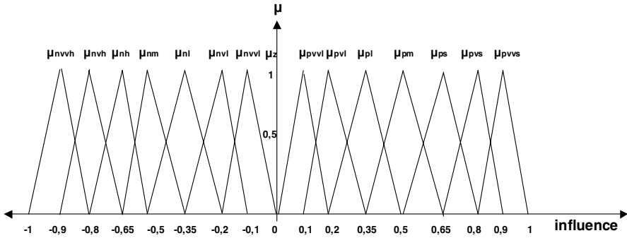
Fig. 3 Membership functions of linguistic variable influence
