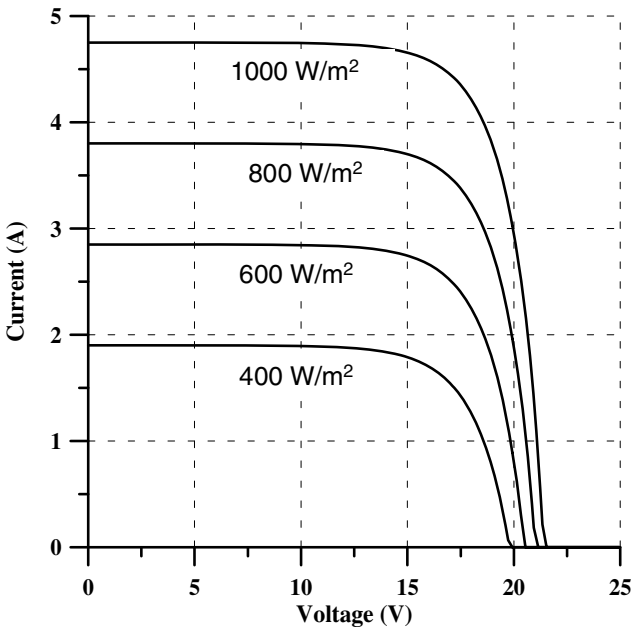
Fig. 2 PV array I-V Characteristics at various insolation levels
