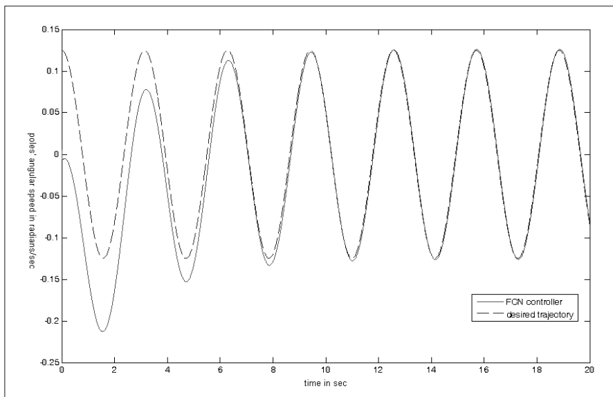
Fig. 17 State x_2(t) and its desired value \frac{\cos(2\pi t)}{8} for initial condition x_1(0) = \pi/8, x_2(0) = 0
