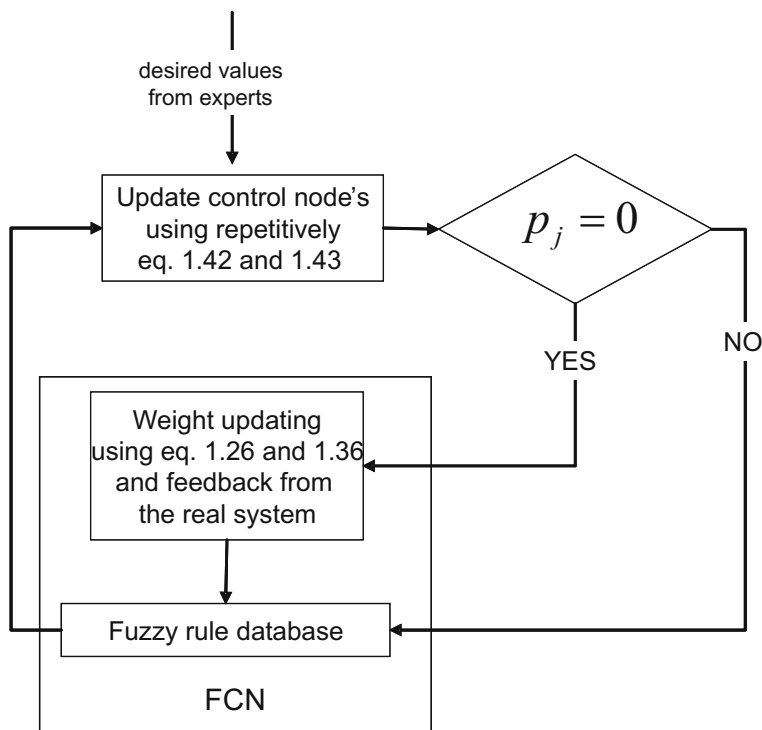
Fig. 25 Control structure in order to achieve the desired equilibrium point defined from the experts
