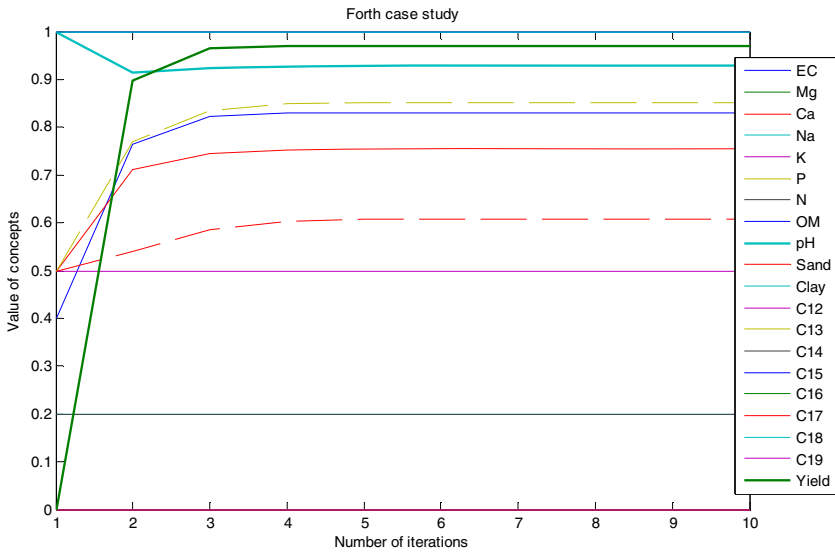
Fig. 11 Subsequent values of concepts for fourth case study till convergence
