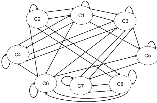
Fig. 1 An FCM with 8 nodes
