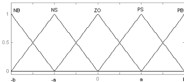
Fig. 5 Membership function for input and output
