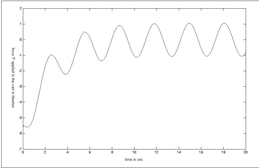
Fig. 18 Force T applied in the cart for tracking state x_1(t) in the desired value \frac{\sin(2*t)}{16} for initial condition x_1(0) = \pi/8 , x_2(0) = 0
