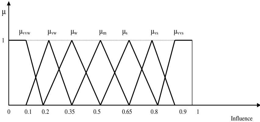
Fig. 2 The 7 membership functions corresponding to each one of the 7 linguistic variables
