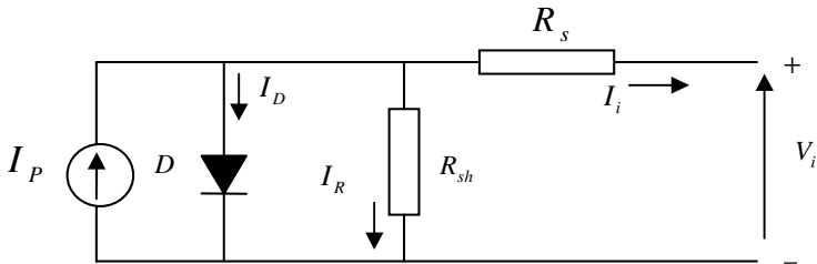
Fig. 4 Equivalent circuit of a solar cell
