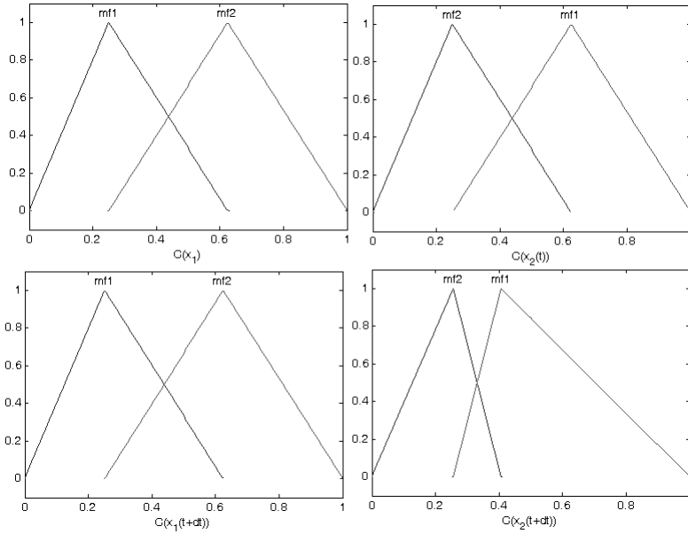
Fig. 12 Left hand side (if-part)
