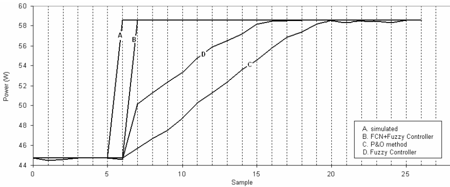
Fig. 15 Sample vs Power of PV-array,
