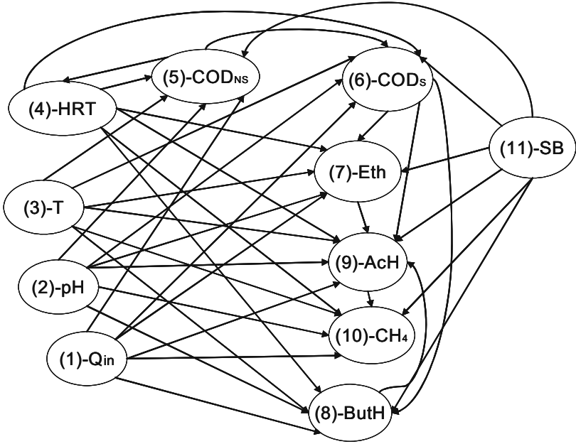
Fig. 23 The FCN designed for the control of the Anaerobic Digestion Process
