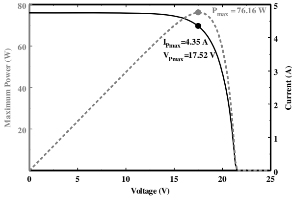
Fig. 1 PV array I-V and P-V Characteristics
