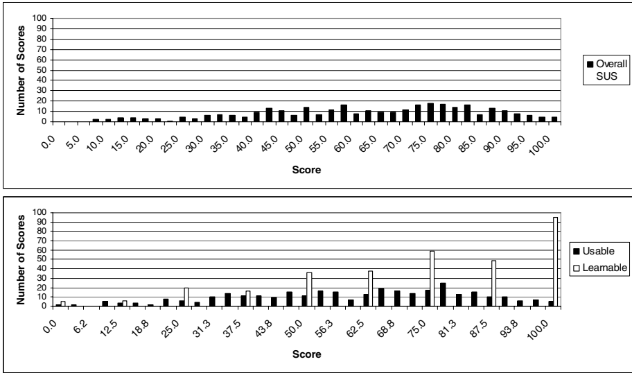
Fig. 2. Distributions of the Overall SUS, Usable, and Learnable scores from the current data set
