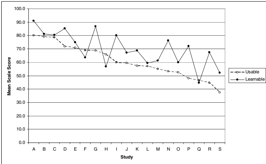
Fig. 1. The Test by Scale interaction
