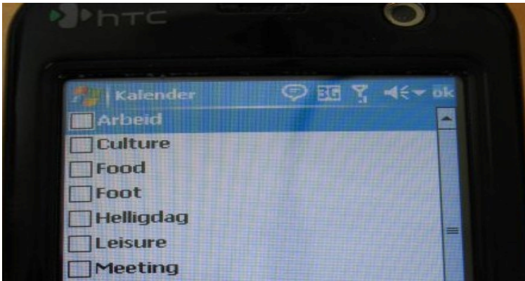
Fig. 1. Taxonomy interface
