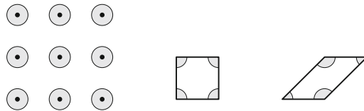
Fig. 15.4 A periodic distribution on \mathbb{Z}^2 (left), restricted \mathcal{P}((0, 1), (1, 0)) (center), and to \mathcal{P}((0, 1), (1, 1)) (right)
