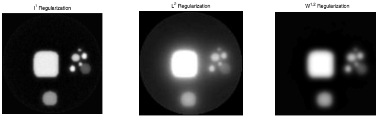
Fig. 3. The above figures are intended to compare our benchmark results to those of other popular methods, e. g., L^2 and W^{1,2} regularization. Here, l^1 , as depicted to the left tends to yield the clearest approximations of the original objects. We have however noticed, that in some cases small peaks may not be preserved during the regularization process. On the other hand, L^2 appears not only slightly more blurred but also fails to remove the circle object caused by the Radon Transform which we consider a major drawback. Finally, W^{1,2} regularization tends to produce strong object blurs which may be a problem not only for small and dense peaks but also deteriorate the overall reconstruction quality.
