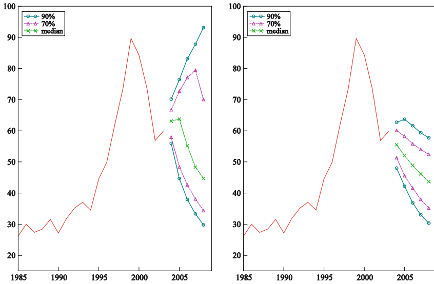
Fig. 7.4 Quantiles of 2,000 simulated predictions of the PD-ratio for the nonlinear evolutionary switching model (left) and the linear, representative agent model (right). Both models are estimated using data until 2003 and then predict up to 5 years ahead
