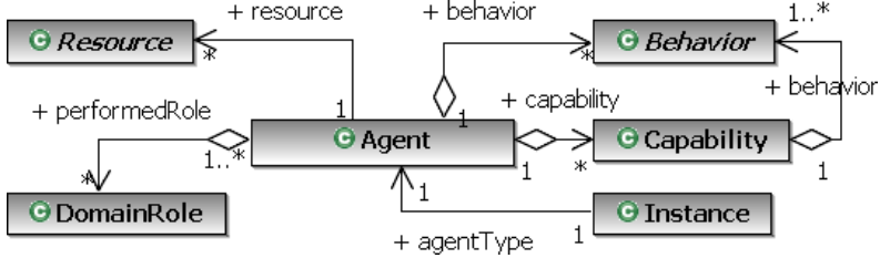
Fig. 3. The metamodel of the agent view
