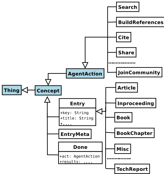
Fig. 3. Interaction ontology of BibFinder
