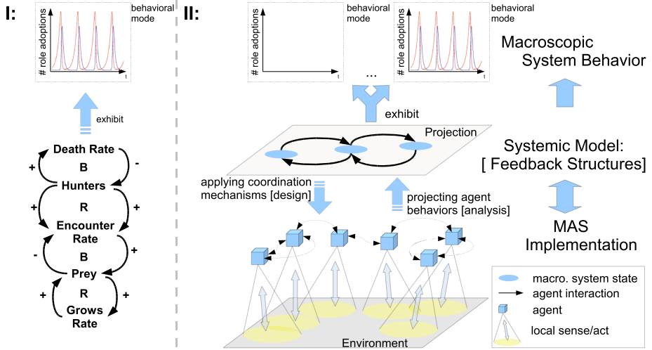
Fig. 1. I: An example CLD. II: MAS implementations can be projected into system dynamics models that describe the causal relations between macroscopic system states
