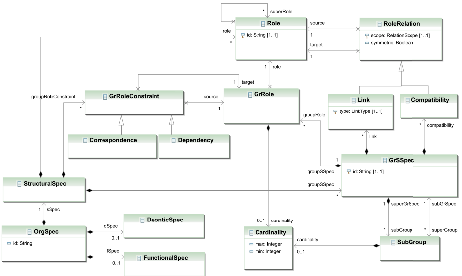
Fig. 2. Merge of AGR and MOISE+
