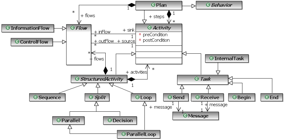
Fig. 6. The partial metamodel of the behavioral view
