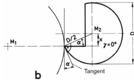
Figure 7.38b Formation of the tool orthogonal clearance for the wheel turning tool. M 1 workpiece centre, M 2 tool centre, D Ø of the formed wheel, x offset in height, \alpha tool orthogonal clearance
