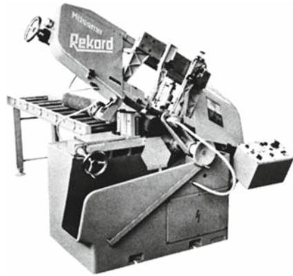
Figure 10.2 Band saw in resting position Type LBU 421 (photo by A. Mössmer, Mutlangen)
