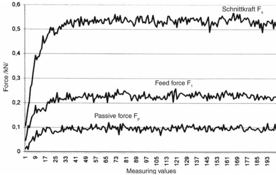
Figure 22.4 Test results for turning k = 70^\circ ; a_p = 2,5 mm; f = 0,112 mm/rev)
