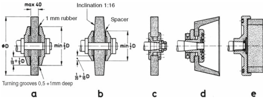
Figure 13.32 Wheel mounting
