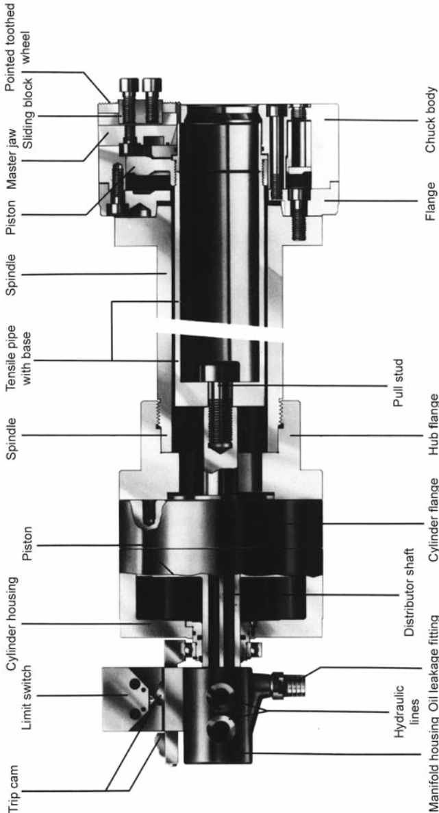
Figure 7.19 Partially hollow chuck: power-actuated chuck with opening, hydraulic full chuck cylinder without opening. (photo by Röhler, Sontheim)
