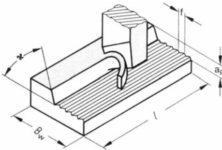
Figure 8.3 Cutting parameters for planing l workpiece length, B_w workpiece width, f feed, a_p depth of cut, \iota tool cutting-edge angle
