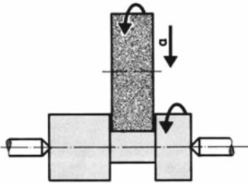
Figure 13.6 Plunge grinding – working principle
