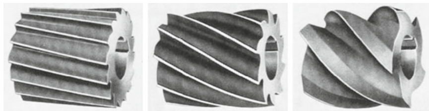
Figure 11.28 Plain milling cutter with key
