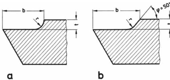
Figure 7.44 Dimensions of chip breaker b in mm width, t in mm depth, r in mm radius, \phi in ^\circ angle of lapping
