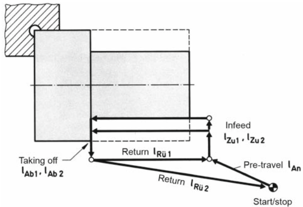
Figure 7.31 Travelling paths in case of automatic procedure
