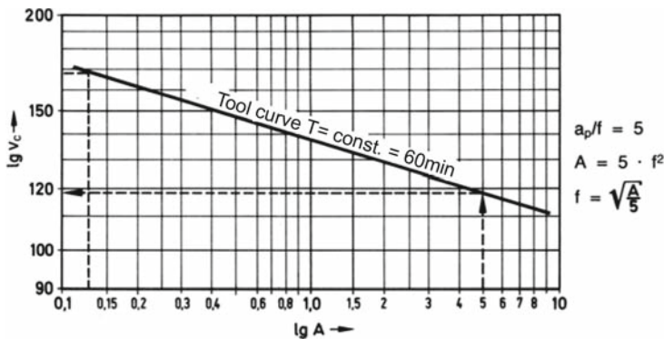
Figure 4.1 Tool curve \lg v_c = f(\lg A) for T = \text{const.}
