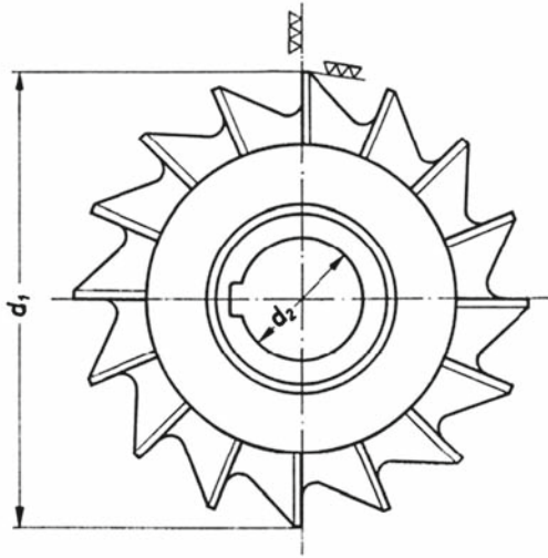
Figure 11.35 Single-angle cutter
