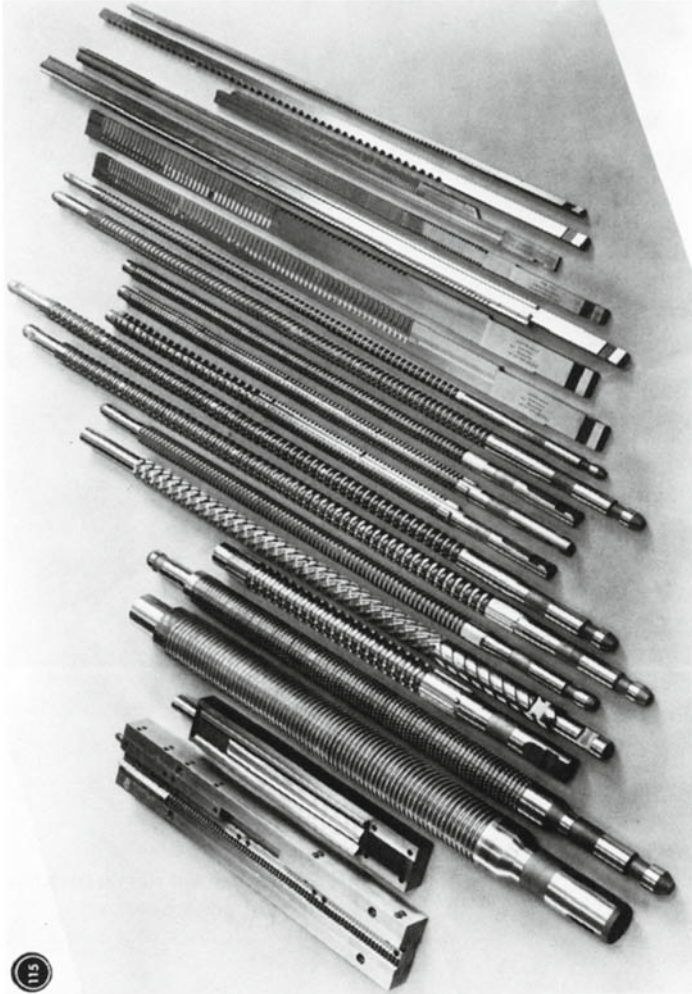
Figure 12.12 Broach types for internal- and external broaching (photo by Karl Klink, Niefern)
