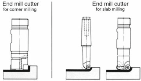
Figure 11.38a End mill cutter tipped with cemented carbide inserts
