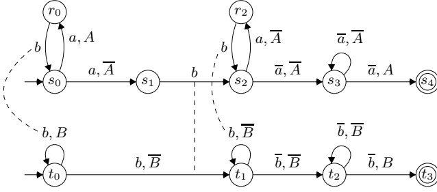
Fig. 1. A concurrent visibly pushdown automaton
