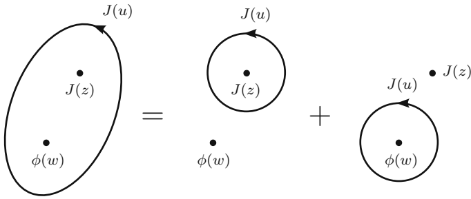
Fig. 4.6 Illustration for the computation of monodromies
