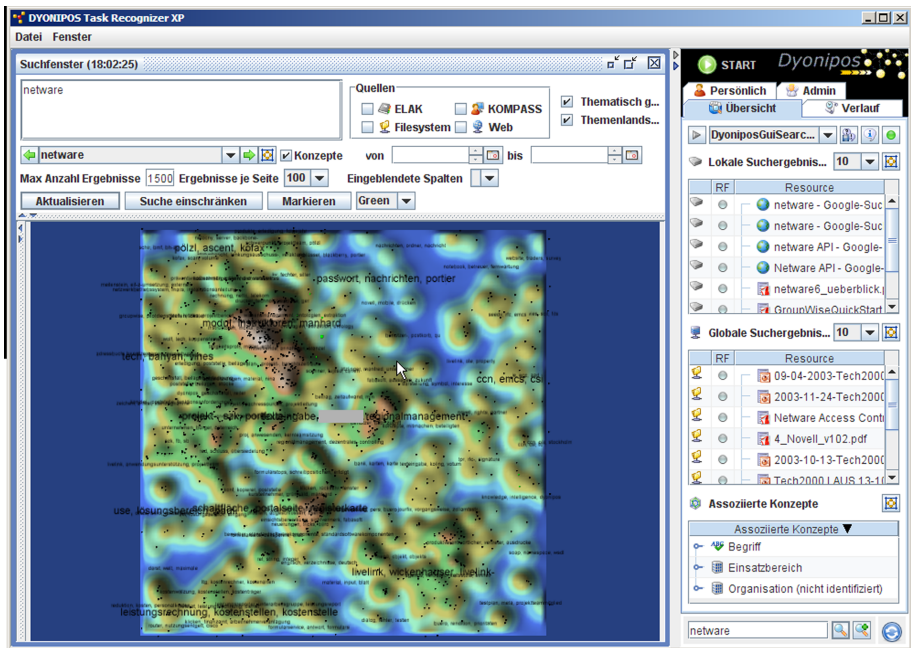
Fig. 3. Visualisation of similar tasks utilising landscape visualisation methods. Similar tasks are placed close to each other generating “islands” of similar tasks. Height indicates the amount of similar tasks. Additionally, islands are labeled with the most frequent keywords and/or persons for the tasks in this island.
