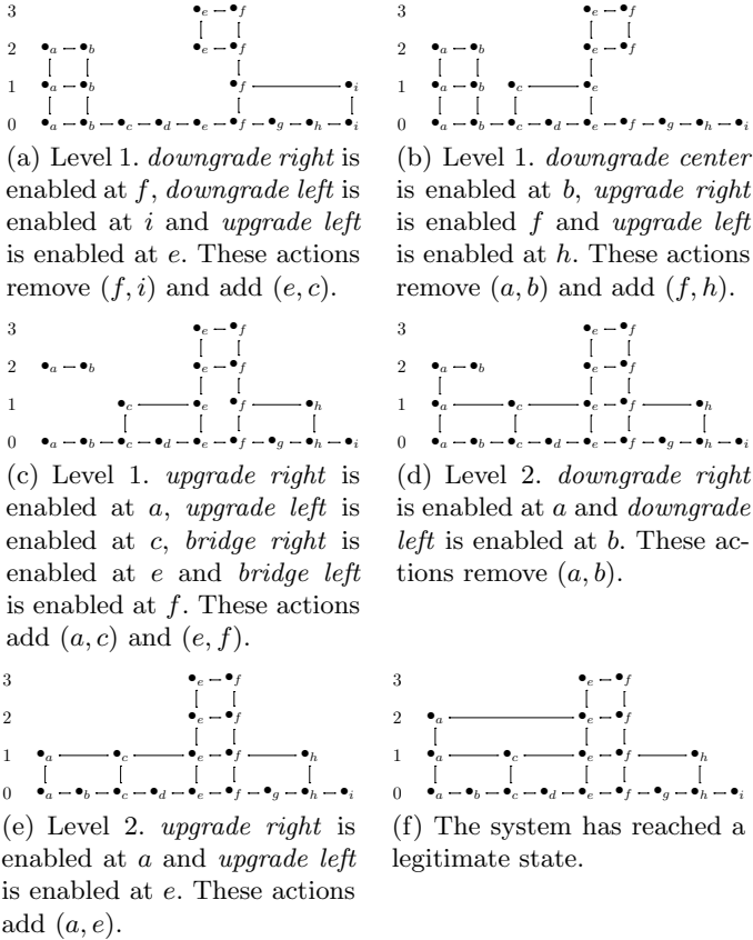
Fig. 6. s-Tiara . We list the processes in the increasing order of their identifiers. b-Tiara has stabilized to \mathcal{GT} . In each state we only mention the enabled actions that are relevant to the discussion. We do not illustrate the operation of prune .
