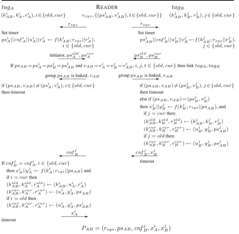
Fig. 3. An anonymous grouping-proof with forward-security—for two tags
