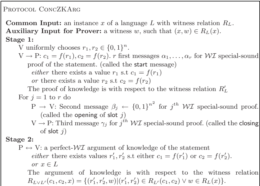
Fig. 1. Concurrent Perfect \mathcal{ZK} argument for \mathcal{NP}
