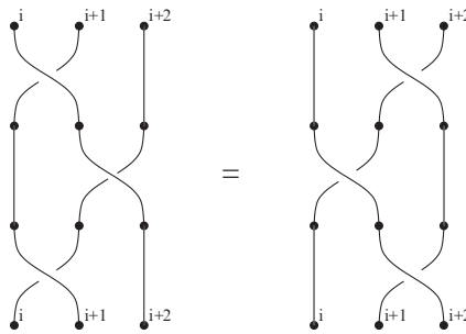
Fig. 6. Relation aba = bab on braids
