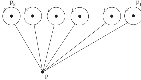
Fig. 7. A geometric basis of \pi_1(\mathbb{C} - \{1, \dots, n\})
