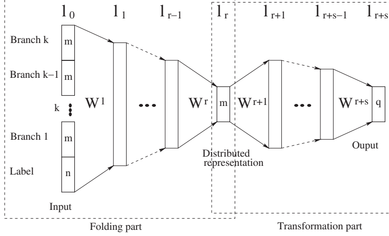
Fig. 1. Kùchler et al. generic folding architecture
