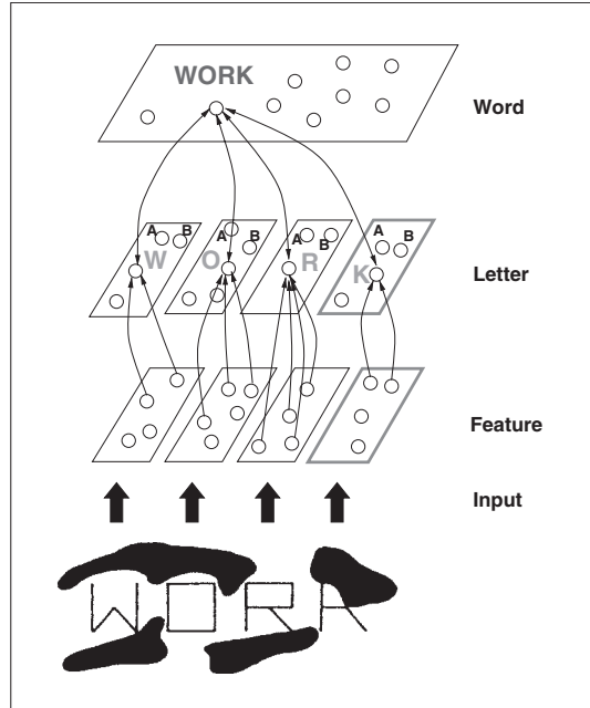
Fig. 5. Côté et al. hierarchically organized ANN model
