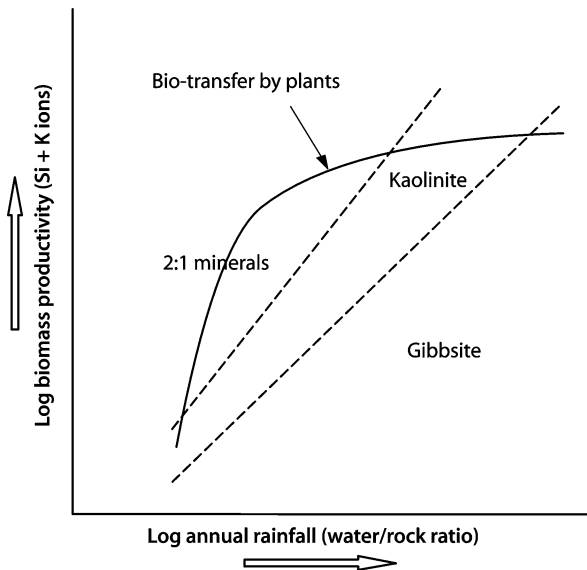
Fig. 8.6. Schematic diagram representing the effect of rainfall on plant activity (biomass) which indicates the amount of material translocated from depth to the surface soil mineral zone. The biomass curve shows that at high rainfall, the plant regime will not exceed a certain amount of translocation effect and hence dissolution of alkalis and silica proceeds producing the kaolinite and eventually gibbsite soil clay assemblages. Lower rainfall shows great changes in biomass, due essentially to the variations of rainfall throughout the year. Steady rainfall gives higher biomass production that does irregular, contrasted season rainfall where biomass production is lower
