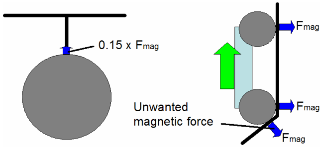
Fig. 2. Obstacles: force decrease on ridges (left); unwanted forces at angular 135° transitions (right)
