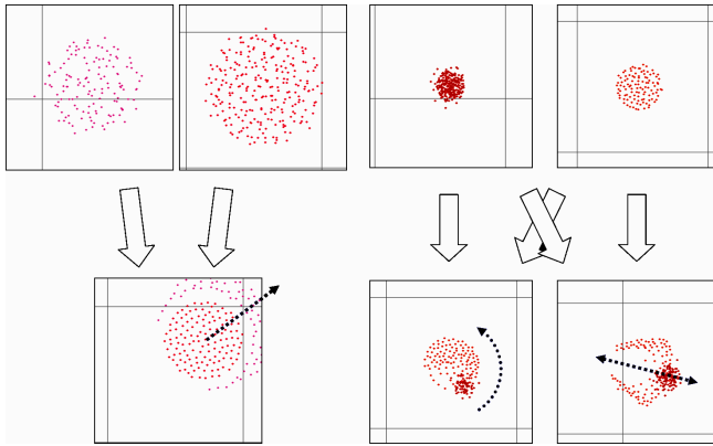
Fig. 3. Production of movements as a result of reaction in Swarm Chemistry. Left: Linear motion. Two originally immobile chemical species form a polarized cluster when blended, and their chasing/escaping behaviors create a linear motion of the entire swarm population. Middle: Rotation. The red cluster rotates around the orange cluster counterclockwise. Right: Linear oscillation. The red cluster is continuously attracted by the orange cloud and keeps moving back and forth through it. In this particular example, the last two movements arise from the same two chemical species. Their relative positions and proportions determine which movement will result.
