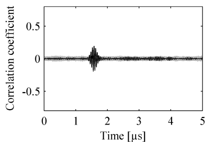
Fig. 6. Result of a DEMA attack on the passively powered prototype inside the reader field
