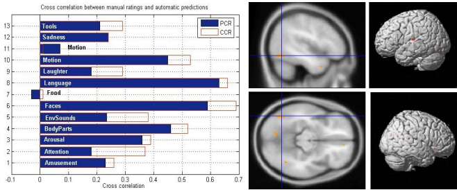
Fig. 1. Left: cross correlation values from cross-validation for 13 core movie features, using principal component analysis (PCR) and canonical correlation analysis (CCR) Right: gray level image with color overlay and surface rendering of a subset of predictive voxels from second level analysis. Color denotes predictive power and cross hair shows most predictive location.
