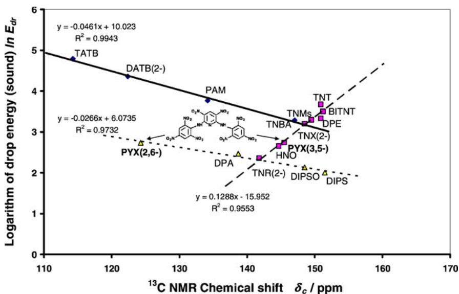
Fig. 12 Relationship between the energy, E_{dr} , (impact sensitivity detected by sound) and ^{13}\text{C} NMR chemical shifts, \delta_c , of the carbon atoms of the aromatic system carrying the most reactive nitro groups (the numbers in brackets denote the positions in the molecule) [165]
