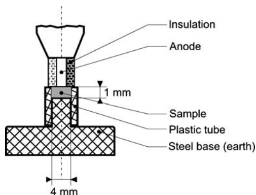
Scheme 5 A spark gap in the ESZ KTTV instrument [8]
