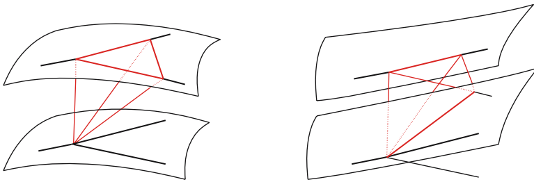
Fig. 9. The Hamiltonian constraint induces a 1 \rightarrow 3 move in the spin foam formalism ( figure on the left ). However, by slicing space-time in a different way, one can equivalently interpret this part of the spin foam as containing a 2 \rightarrow 2 move ( figure on the right ). This argument suggests that the ultra-local Hamiltonian may not be sufficient to achieve space-time covariance. For clarity, the network edges which lie in one of the spatial slices have been drawn as thick lines
