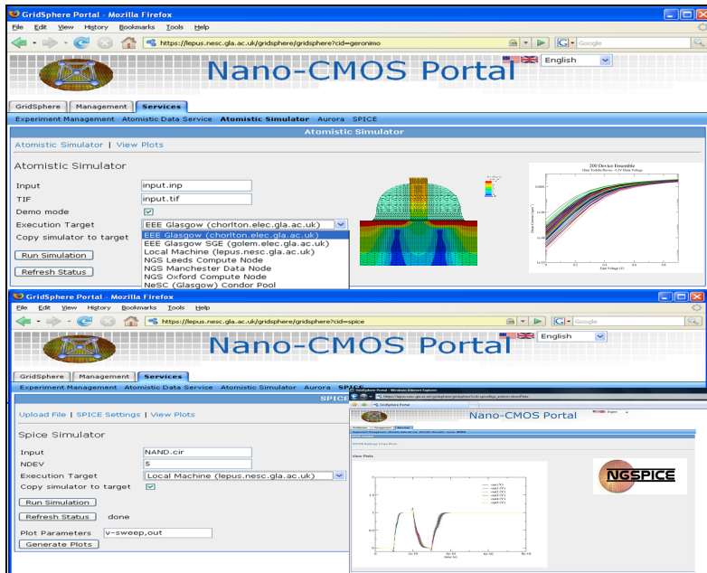
Fig. 1. Atomistic Device Modeling Service and I/V Outputs (above) and Circuit Simulation of NAND gate incorporating atomistic variability (below)
