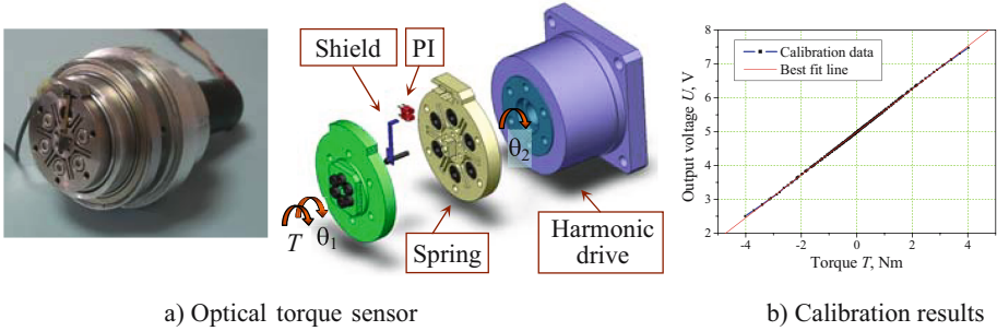
Fig. 2. Torque sensor of the elbow joint and calibration results
