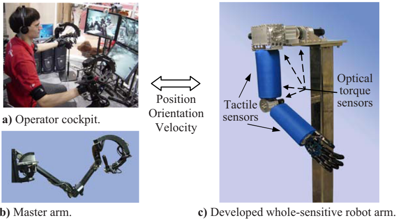
Fig. 1. Robot teleoperation system
