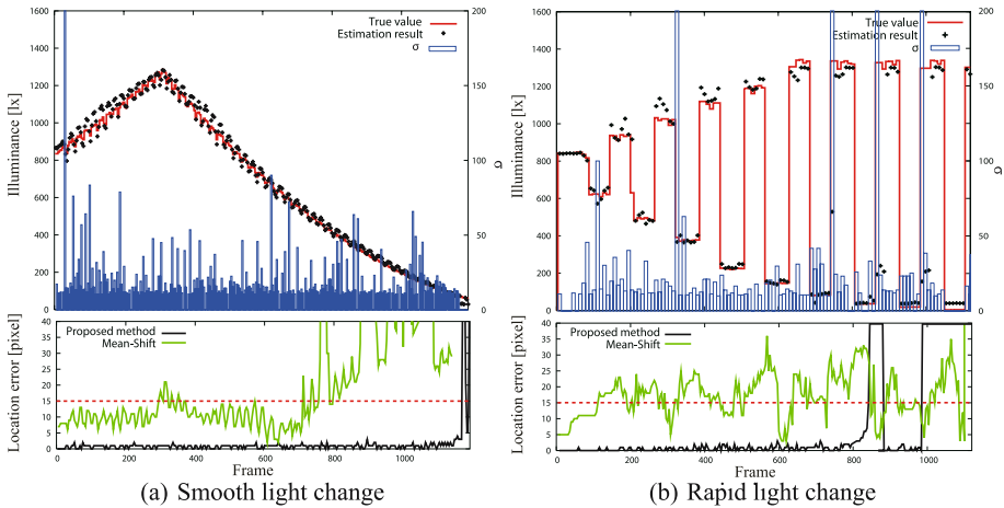
Fig. 6. Experimental results
