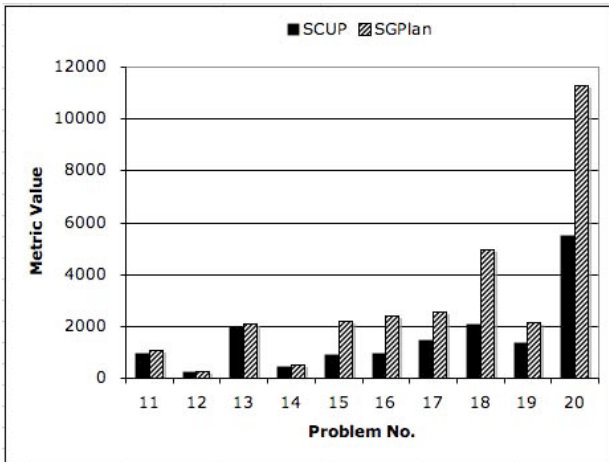
Fig. 4. The violation costs of the solutions generated by SCUP and SGPlan on the larger Rover problems
