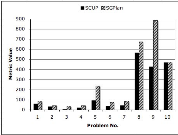
Fig. 3. The violation costs of the solutions generated by SCUP and SGPlan on the smaller Rover problems
