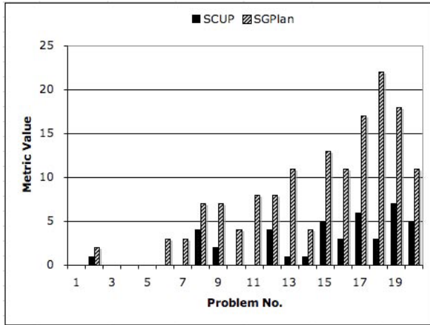
Fig. 2. The violation costs of the solutions generated by SCUP and SGPlan on the Trucks problems
