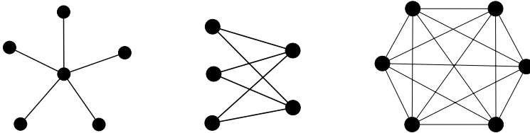
Fig. 9.1. Star (left), complete bipartite graph (middle) and complete graph (right)
