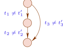
Fig. 2. Boolean combinations of guards.
