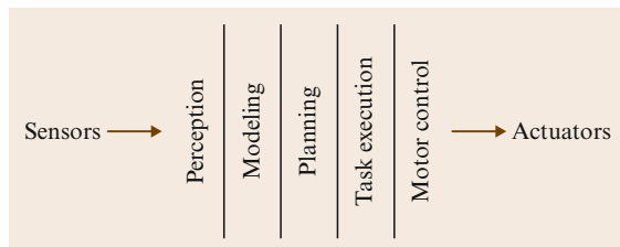
Fig. 8.2 The sense–plan–act (SPA) paradigm (after [8.3], with permission)
