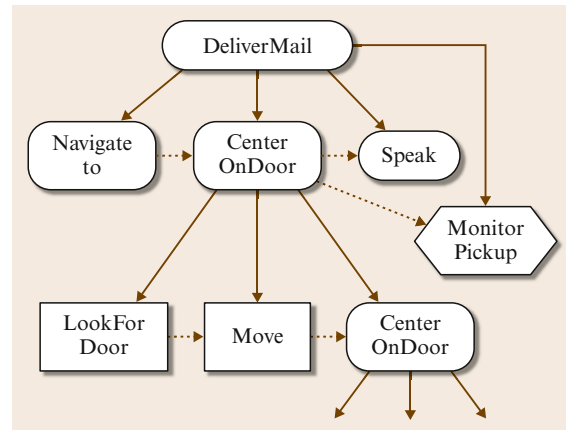
Fig. 8.8 Hierarchical task tree for mail-delivery task ( lozenge nodes are interior; rectangular nodes are leaves; hexagonal node is an execution monitor; solid arrows are parent–child relationships; dashed arrows are sequential constraints)
